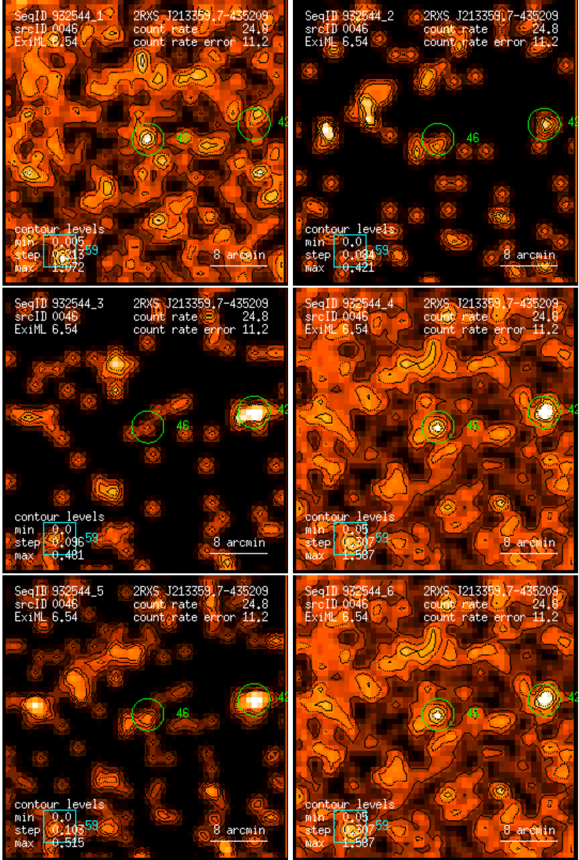
Figure 46: RASS 932544: detection 0046: band rate images, Gaussian filter: (1) PSPC channels 11 – 41, (2) 52 – 90, (3) 91 – 201, (4) 11 – 235, (5) 52 – 201, (6) 11 – 201. Broad band rates in counts/ks. Band rate contour levels in counts/ks/arcmin 2 .
