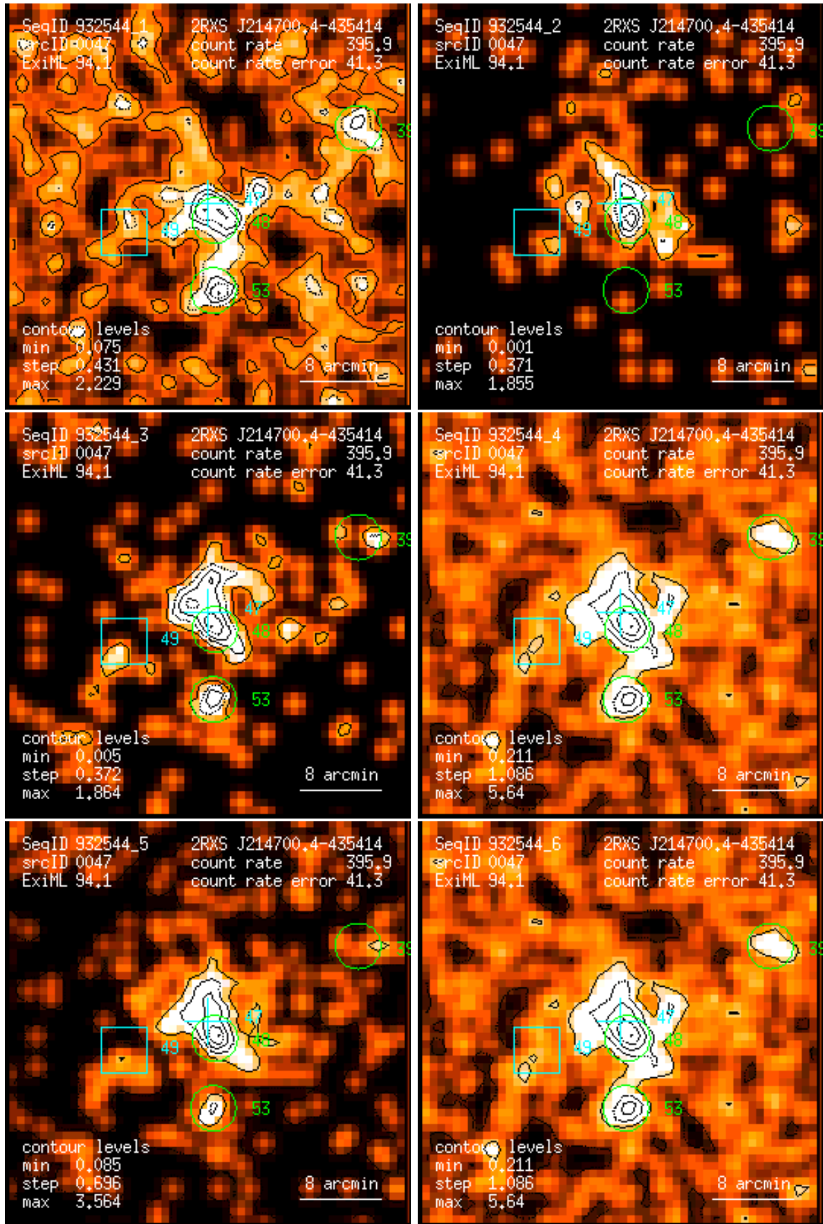
Figure 47: RASS 932544: detection 0047: band rate images, Gaussian filter: (1) PSPC channels 11 – 41, (2) 52 – 90, (3) 91 – 201, (4) 11 – 235, (5) 52 – 201, (6) 11 – 201. Broad band rates in counts/ks. Band rate contour levels in counts/ks/arcmin 2 .
