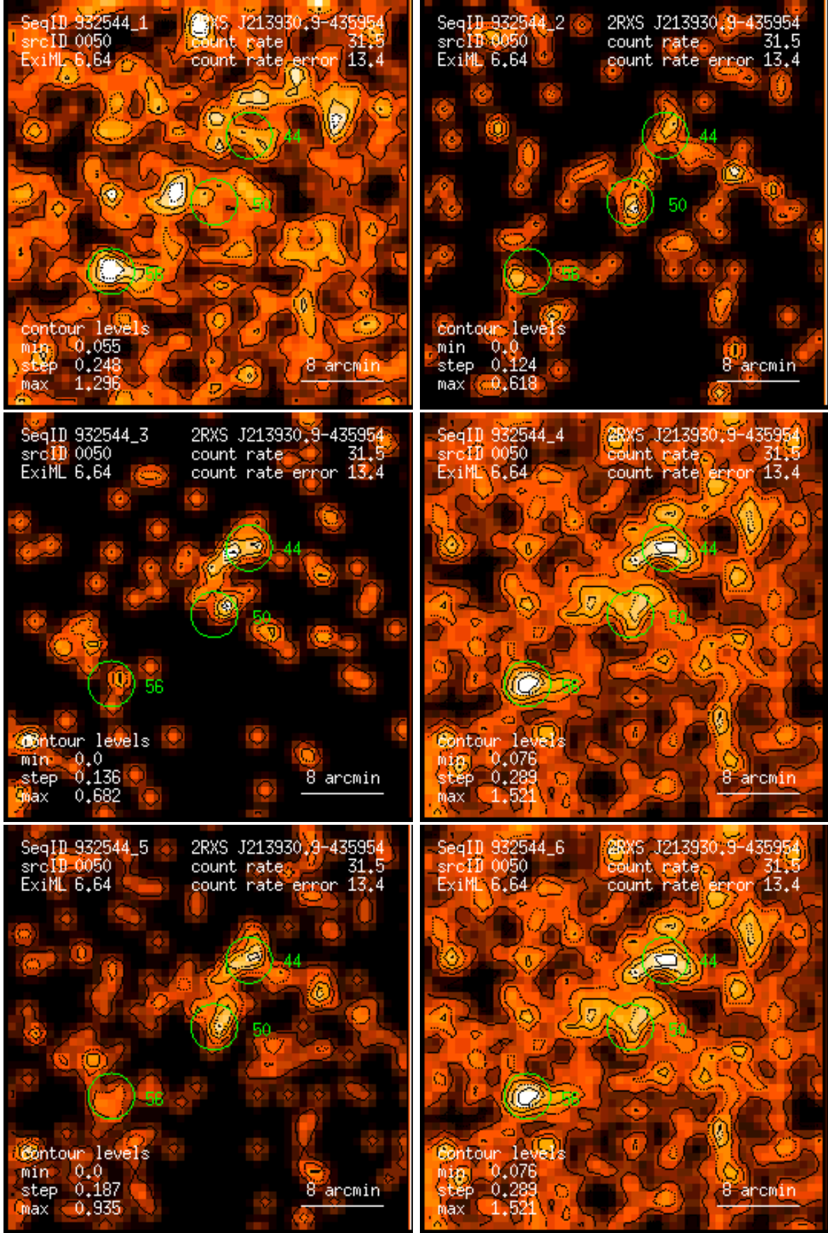
Figure 50: RASS 932544: detection 0050: band rate images, Gaussian filter: (1) PSPC channels 11 – 41, (2) 52 – 90, (3) 91 – 201, (4) 11 – 235, (5) 52 – 201, (6) 11 – 201. Broad band rates in counts/ks. Band rate contour levels in counts/ks/arcmin 2 .
