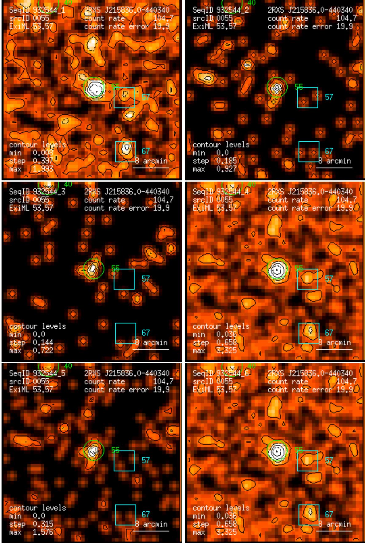
Figure 55: RASS 932544: detection 0055: band rate images, Gaussian filter: (1) PSPC channels 11 – 41, (2) 52 – 90, (3) 91 – 201, (4) 11 – 235, (5) 52 – 201, (6) 11 – 201. Broad band rates in counts/ks. Band rate contour levels in counts/ks/arcmin 2 .
