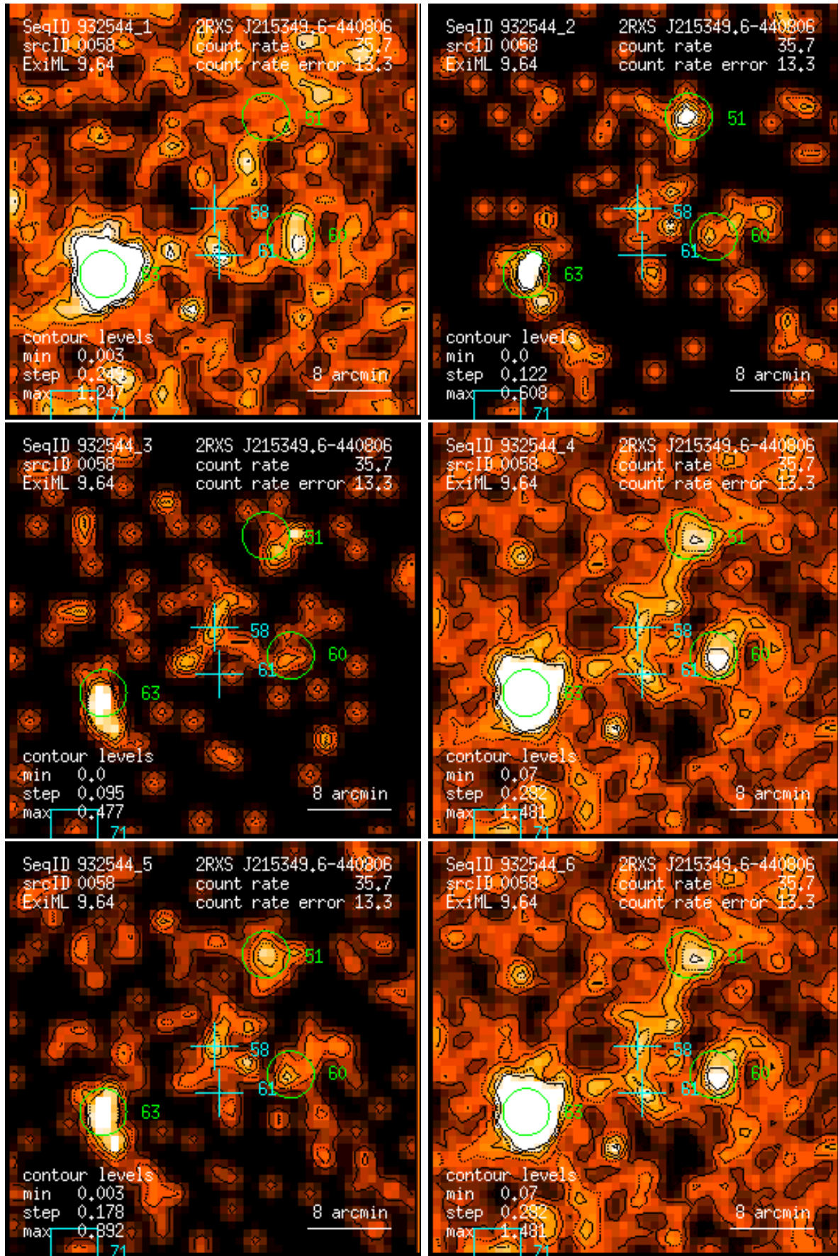
Figure 58: RASS 932544: detection 0058: band rate images, Gaussian filter: (1) PSPC channels 11 – 41, (2) 52 – 90, (3) 91 – 201, (4) 11 – 235, (5) 52 – 201, (6) 11 – 201. Broad band rates in counts/ks. Band rate contour levels in counts/ks/arcmin 2 .
