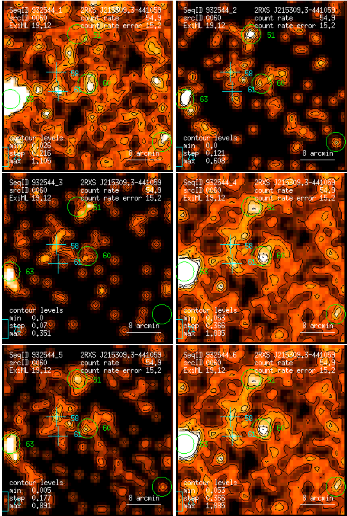
Figure 60: RASS 932544: detection 0060: band rate images, Gaussian filter: (1) PSPC channels 11 – 41, (2) 52 – 90, (3) 91 – 201, (4) 11 – 235, (5) 52 – 201, (6) 11 – 201. Broad band rates in counts/ks. Band rate contour levels in counts/ks/arcmin 2 .
