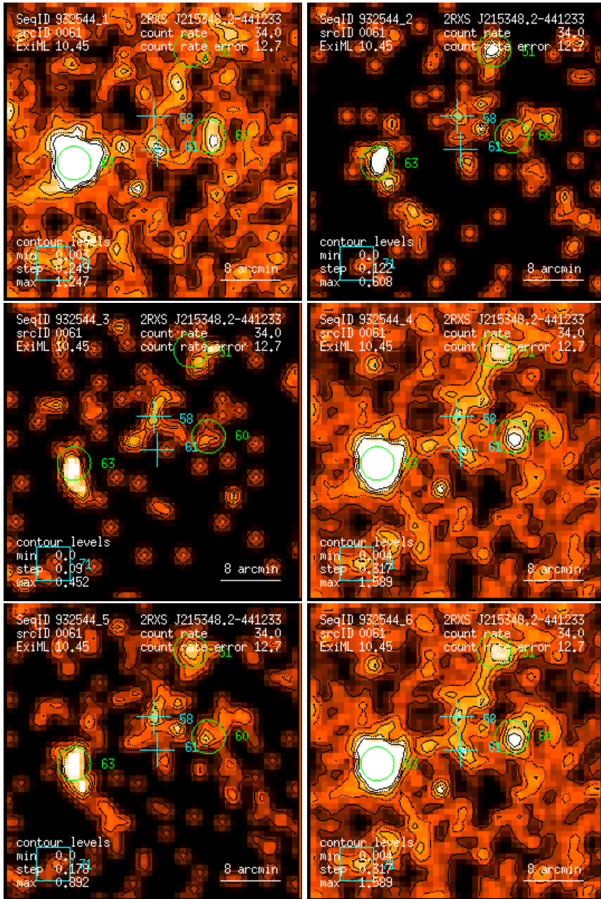
Figure 61: RASS 932544: detection 0061: band rate images, Gaussian filter: (1) PSPC channels 11 – 41, (2) 52 – 90, (3) 91 – 201, (4) 11 – 235, (5) 52 – 201, (6) 11 – 201. Broad band rates in counts/ks. Band rate contour levels in counts/ks/arcmin 2 .
