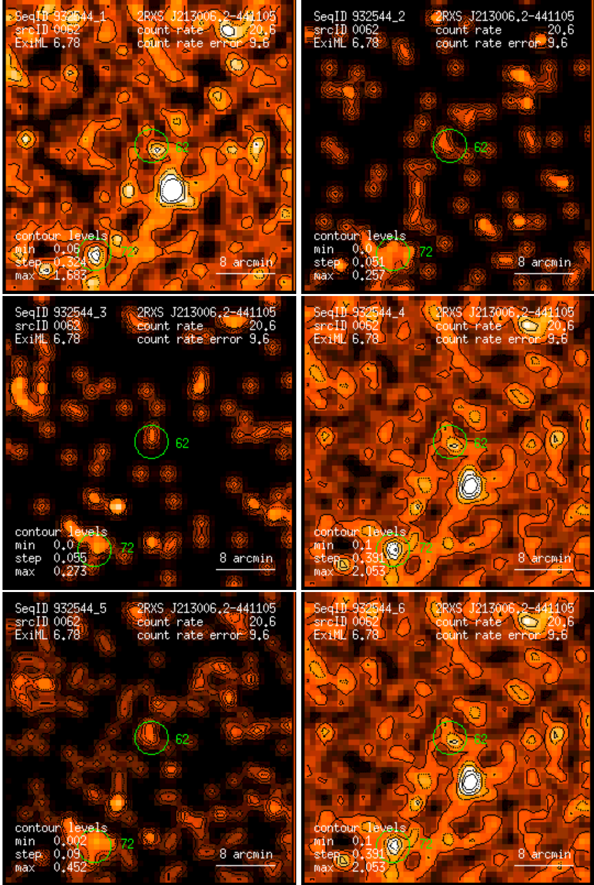
Figure 62: RASS 932544: detection 0062: band rate images, Gaussian filter: (1) PSPC channels 11 – 41, (2) 52 – 90, (3) 91 – 201, (4) 11 – 235, (5) 52 – 201, (6) 11 – 201. Broad band rates in counts/ks. Band rate contour levels in counts/ks/arcmin 2 .
