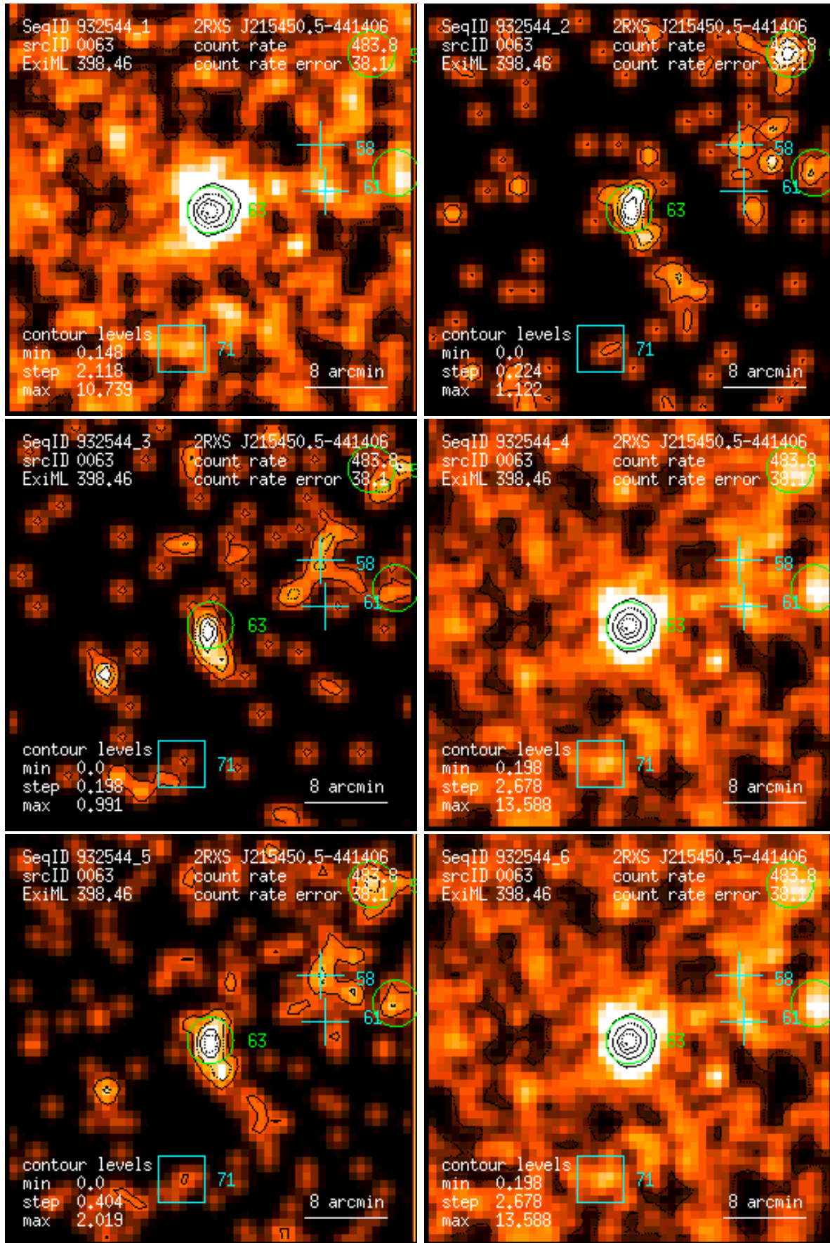
Figure 63: RASS 932544: detection 0063: band rate images, Gaussian filter: (1) PSPC channels 11 – 41, (2) 52 – 90, (3) 91 – 201, (4) 11 – 235, (5) 52 – 201, (6) 11 – 201. Broad band rates in counts/ks. Band rate contour levels in counts/ks/arcmin 2 .
