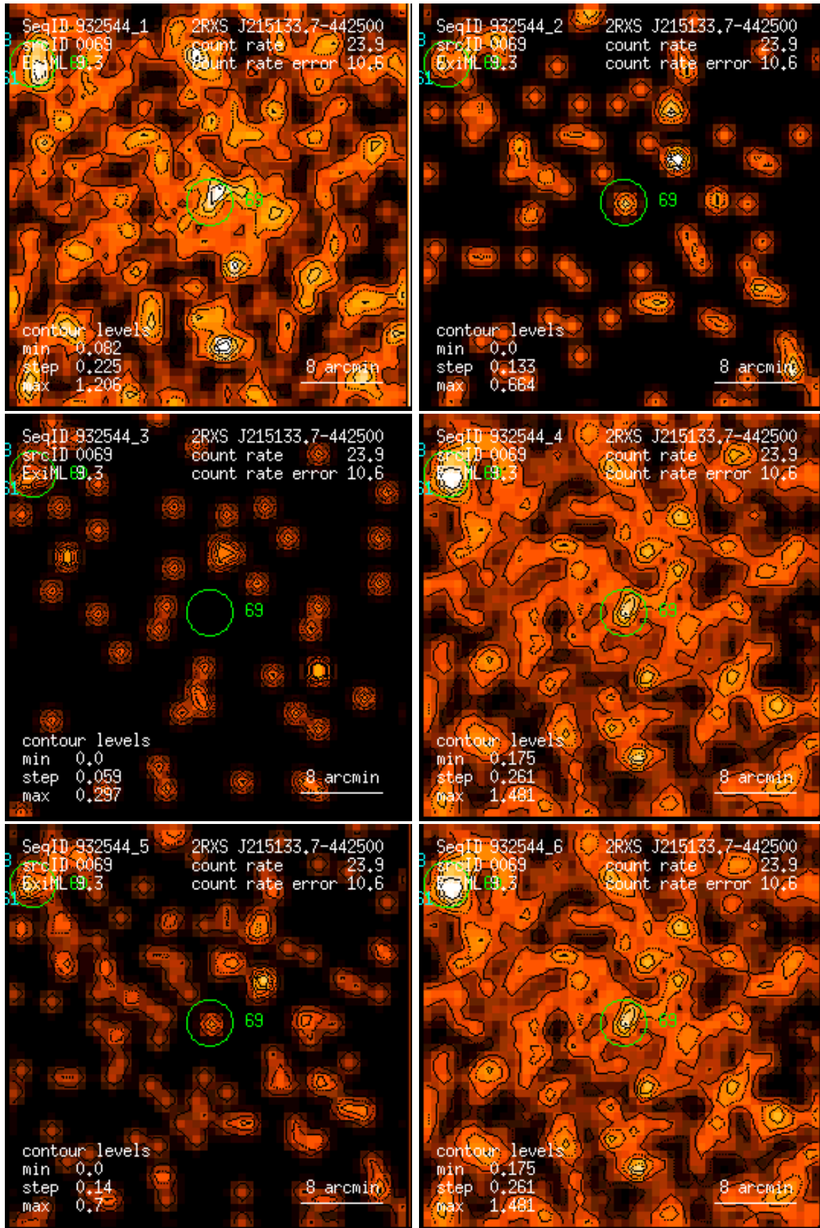
Figure 69: RASS 932544: detection 0069: band rate images, Gaussian filter: (1) PSPC channels 11 – 41, (2) 52 – 90, (3) 91 – 201, (4) 11 – 235, (5) 52 – 201, (6) 11 – 201. Broad band rates in counts/ks. Band rate contour levels in counts/ks/arcmin 2 .
