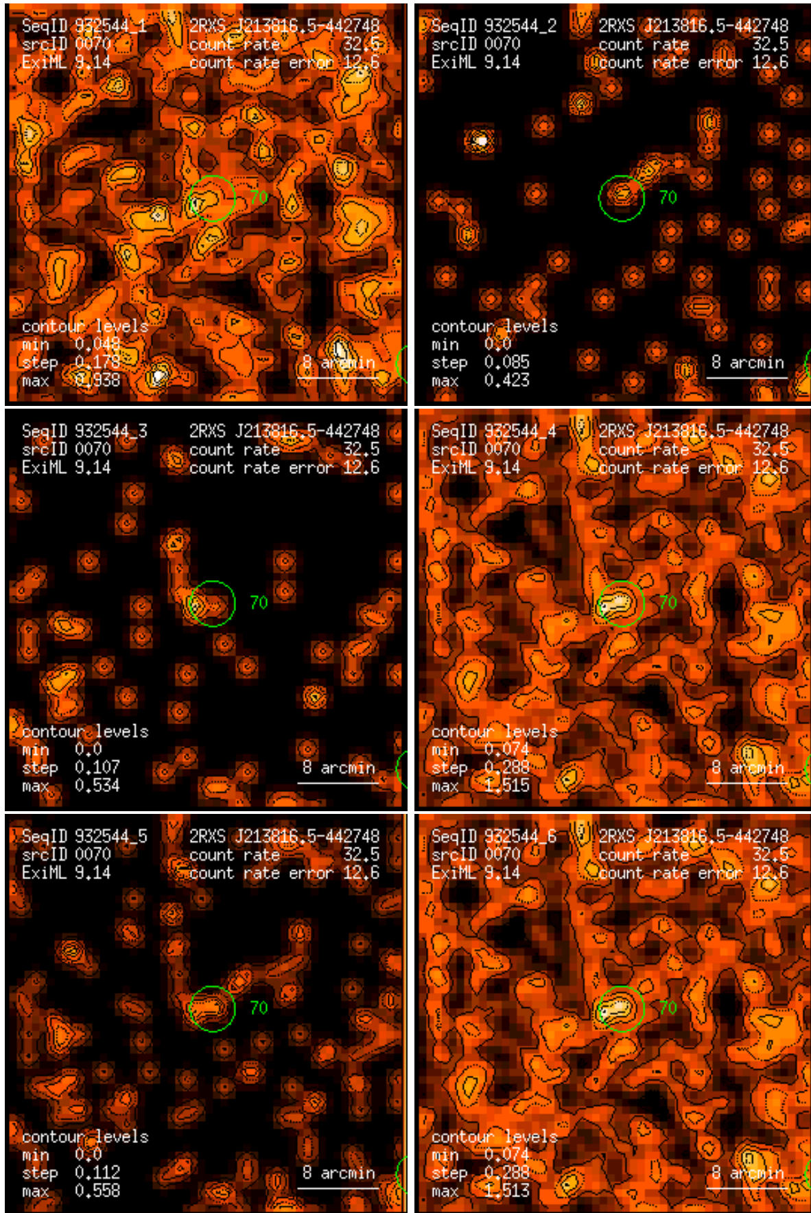
Figure 70: RASS 932544: detection 0070: band rate images, Gaussian filter: (1) PSPC channels 11 – 41, (2) 52 – 90, (3) 91 – 201, (4) 11 – 235, (5) 52 – 201, (6) 11 – 201. Broad band rates in counts/ks. Band rate contour levels in counts/ks/arcmin 2 .
