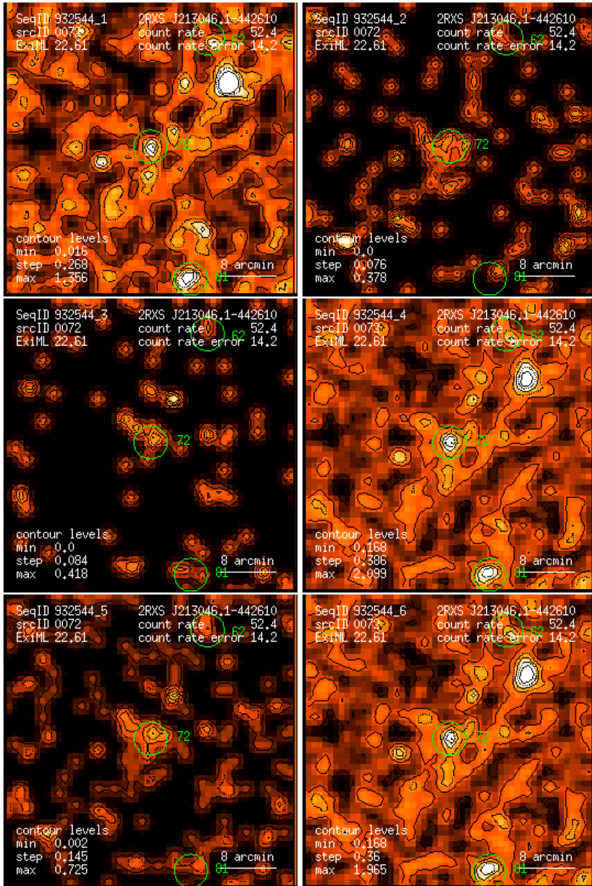
Figure 72: RASS 932544: detection 0072: band rate images, Gaussian filter: (1) PSPC channels 11 – 41, (2) 52 – 90, (3) 91 – 201, (4) 11 – 235, (5) 52 – 201, (6) 11 – 201. Broad band rates in counts/ks. Band rate contour levels in counts/ks/arcmin 2 .
