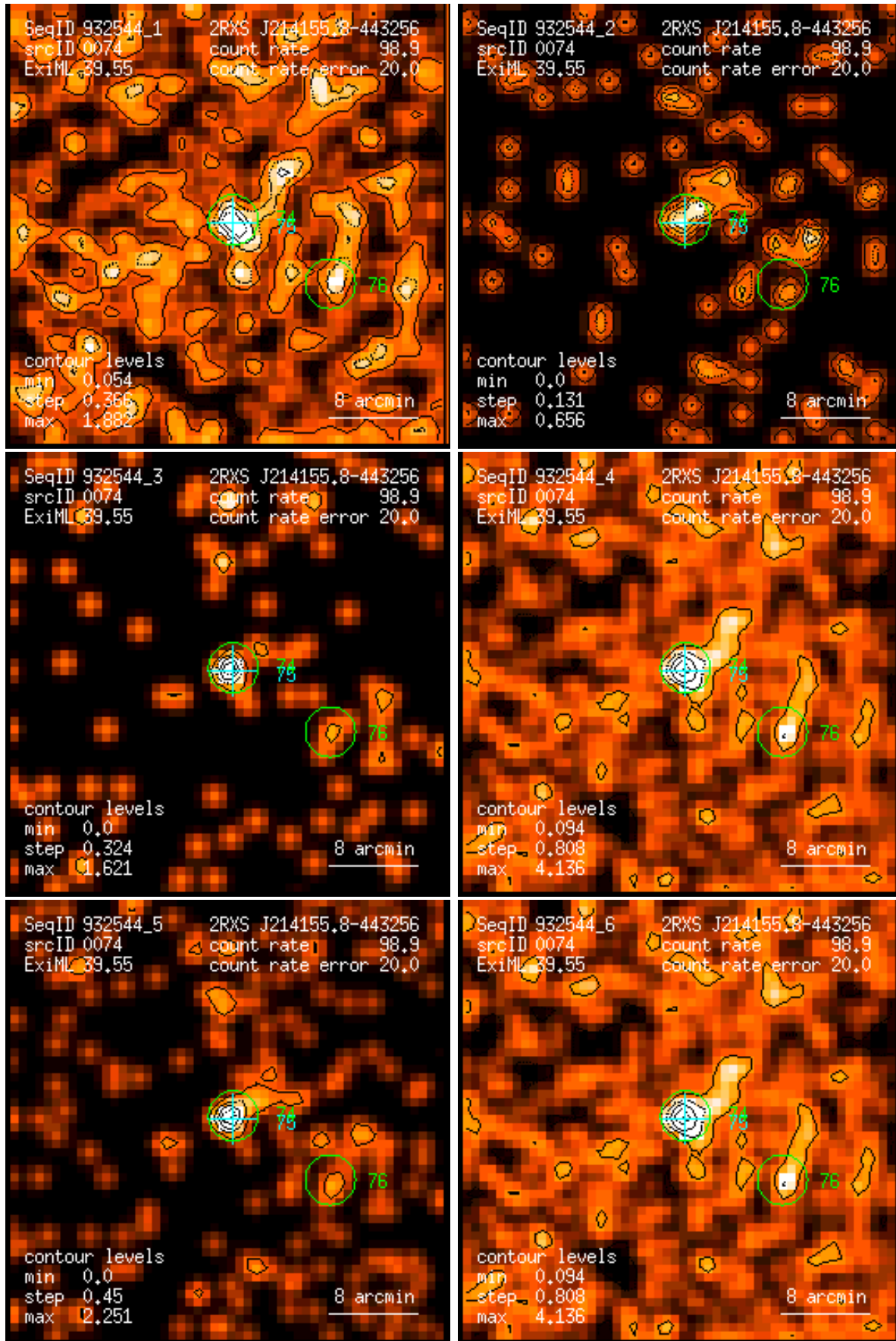
Figure 74: RASS 932544: detection 0074: band rate images, Gaussian filter: (1) PSPC channels 11 – 41, (2) 52 – 90, (3) 91 – 201, (4) 11 – 235, (5) 52 – 201, (6) 11 – 201. Broad band rates in counts/ks. Band rate contour levels in counts/ks/arcmin 2 .
