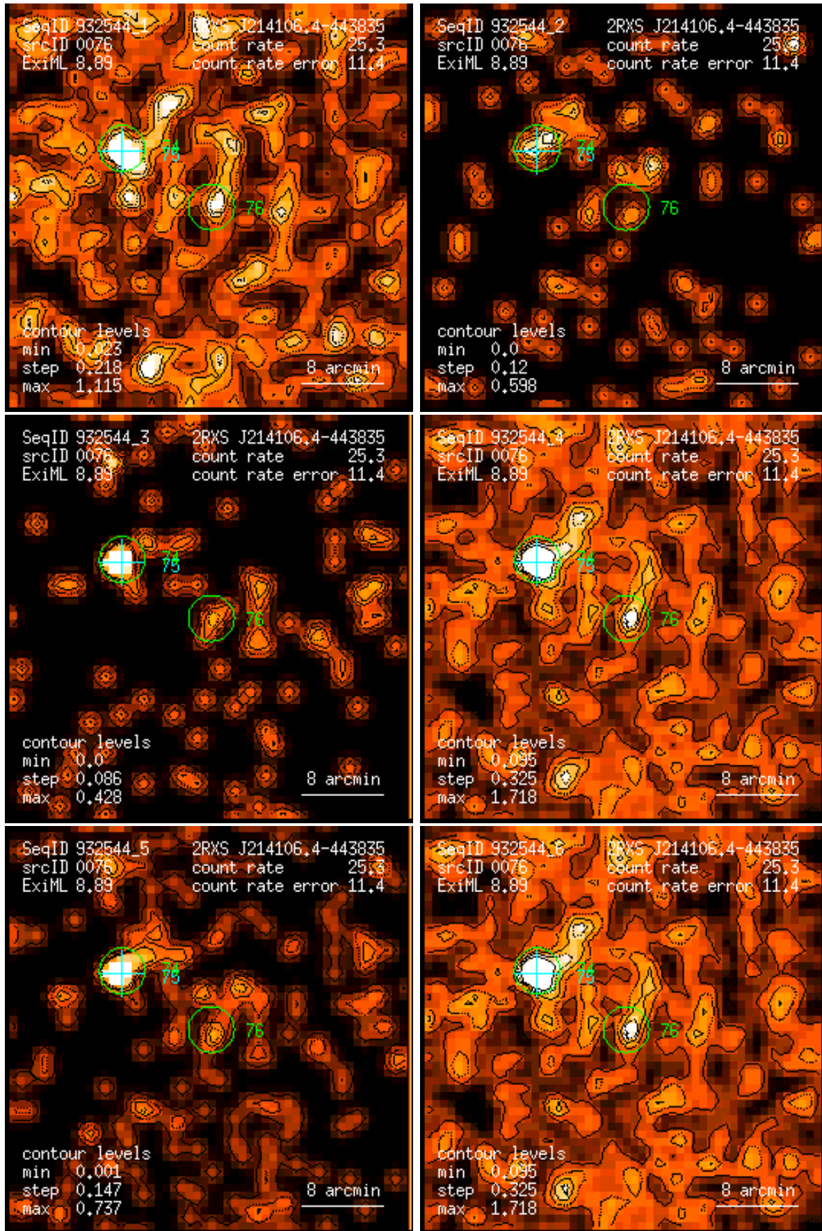
Figure 76: RASS 932544: detection 0076: band rate images, Gaussian filter: (1) PSPC channels 11 – 41, (2) 52 – 90, (3) 91 – 201, (4) 11 – 235, (5) 52 – 201, (6) 11 – 201. Broad band rates in counts/ks. Band rate contour levels in counts/ks/arcmin 2 .
