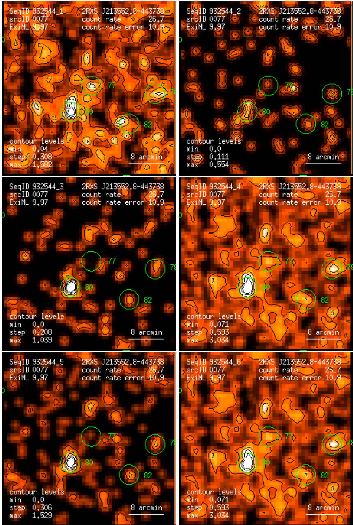
Figure 77: RASS 932544: detection 0077: band rate images, Gaussian filter: (1) PSPC channels 11 – 41, (2) 52 – 90, (3) 91 – 201, (4) 11 – 235, (5) 52 – 201, (6) 11 – 201. Broad band rates in counts/ks. Band rate contour levels in counts/ks/arcmin 2 .
