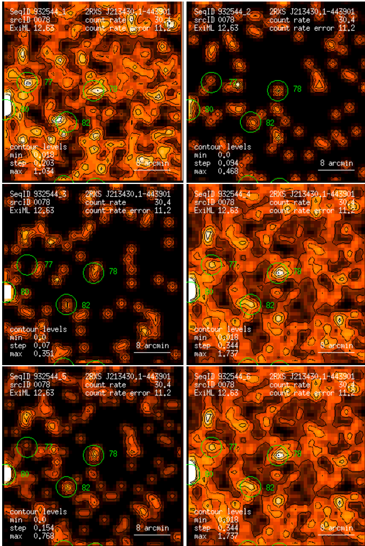
Figure 78: RASS 932544: detection 0078: band rate images, Gaussian filter: (1) PSPC channels 11 – 41, (2) 52 – 90, (3) 91 – 201, (4) 11 – 235, (5) 52 – 201, (6) 11 – 201. Broad band rates in counts/ks. Band rate contour levels in counts/ks/arcmin 2 .
