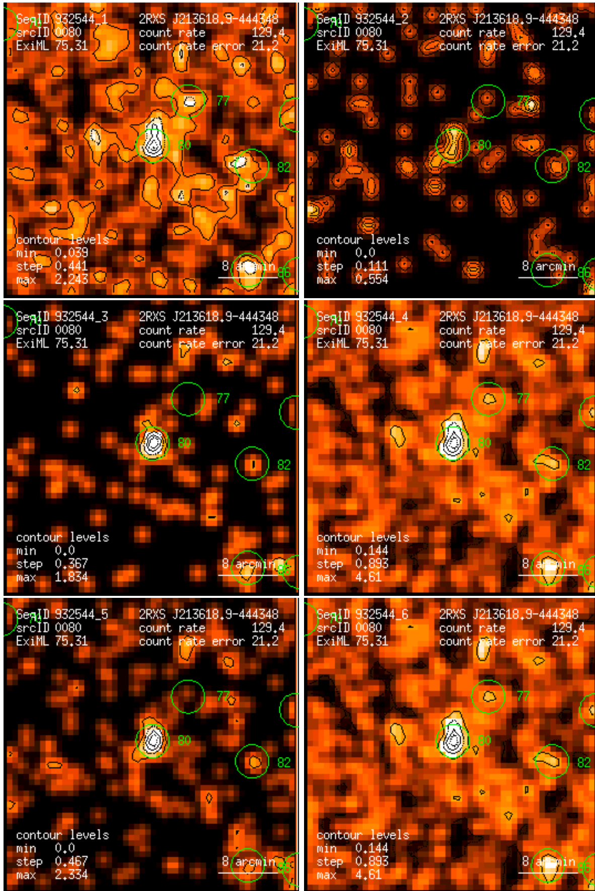
Figure 80: RASS 932544: detection 0080: band rate images, Gaussian filter: (1) PSPC channels 11 – 41, (2) 52 – 90, (3) 91 – 201, (4) 11 – 235, (5) 52 – 201, (6) 11 – 201. Broad band rates in counts/ks. Band rate contour levels in counts/ks/arcmin 2 .
