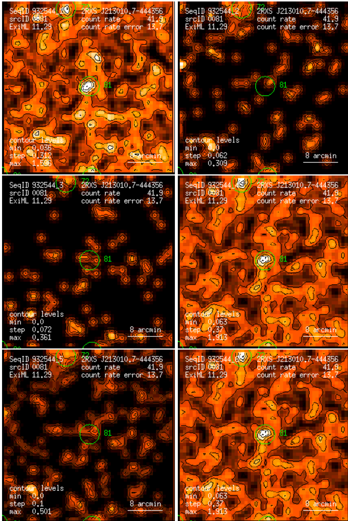
Figure 81: RASS 932544: detection 0081: band rate images, Gaussian filter: (1) PSPC channels 11 – 41, (2) 52 – 90, (3) 91 – 201, (4) 11 – 235, (5) 52 – 201, (6) 11 – 201. Broad band rates in counts/ks. Band rate contour levels in counts/ks/arcmin 2 .
