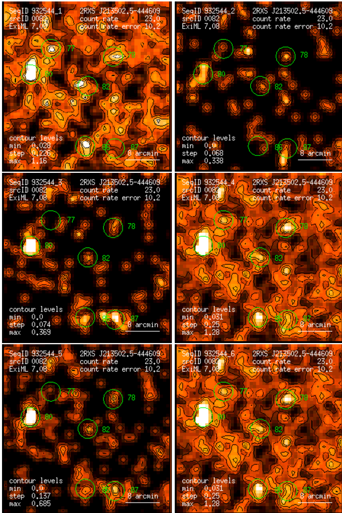
Figure 82: RASS 932544: detection 0082: band rate images, Gaussian filter: (1) PSPC channels 11 – 41, (2) 52 – 90, (3) 91 – 201, (4) 11 – 235, (5) 52 – 201, (6) 11 – 201. Broad band rates in counts/ks. Band rate contour levels in counts/ks/arcmin 2 .
