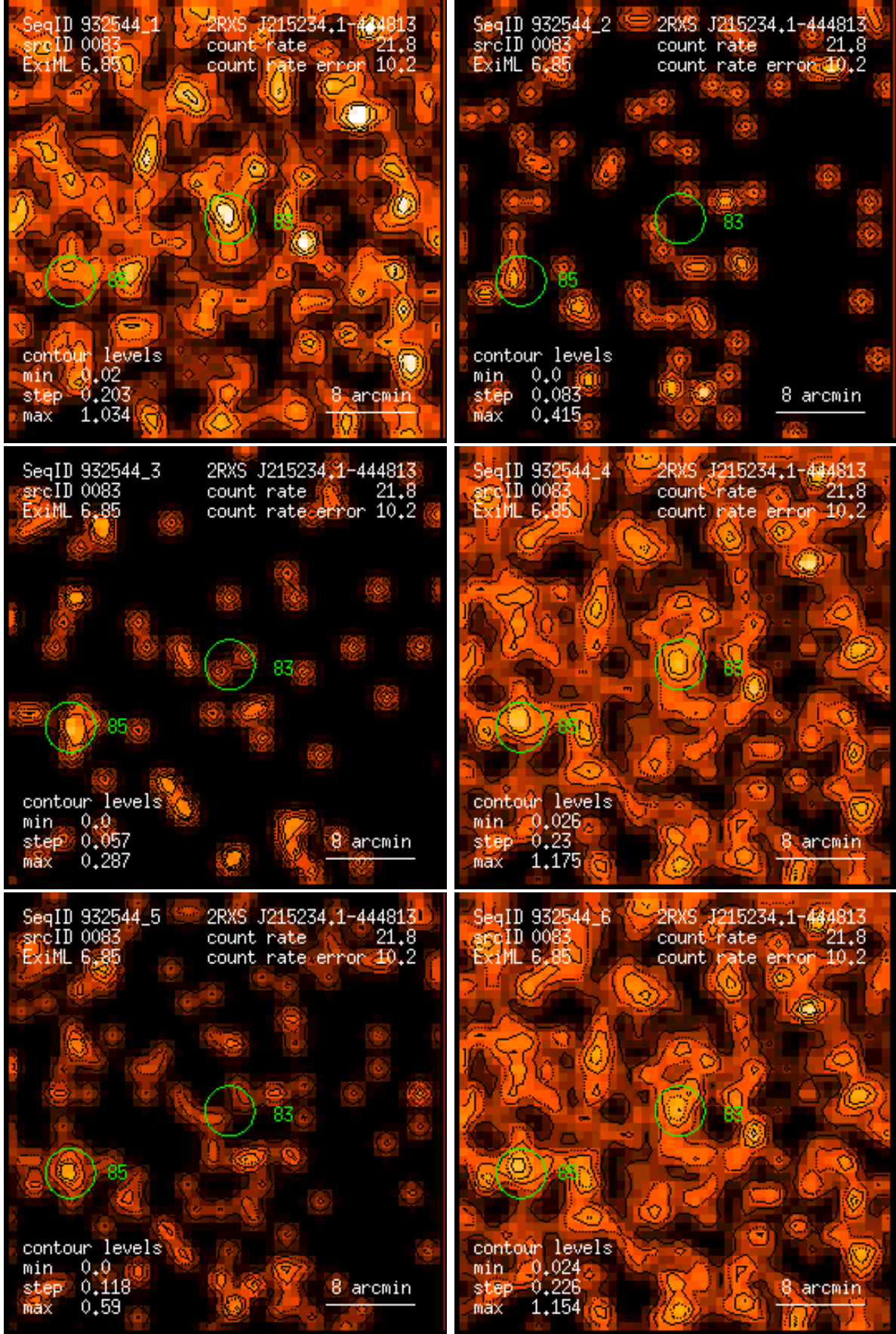
Figure 83: RASS 932544: detection 0083: band rate images, Gaussian filter: (1) PSPC channels 11 – 41, (2) 52 – 90, (3) 91 – 201, (4) 11 – 235, (5) 52 – 201, (6) 11 – 201. Broad band rates in counts/ks. Band rate contour levels in counts/ks/arcmin 2 .
