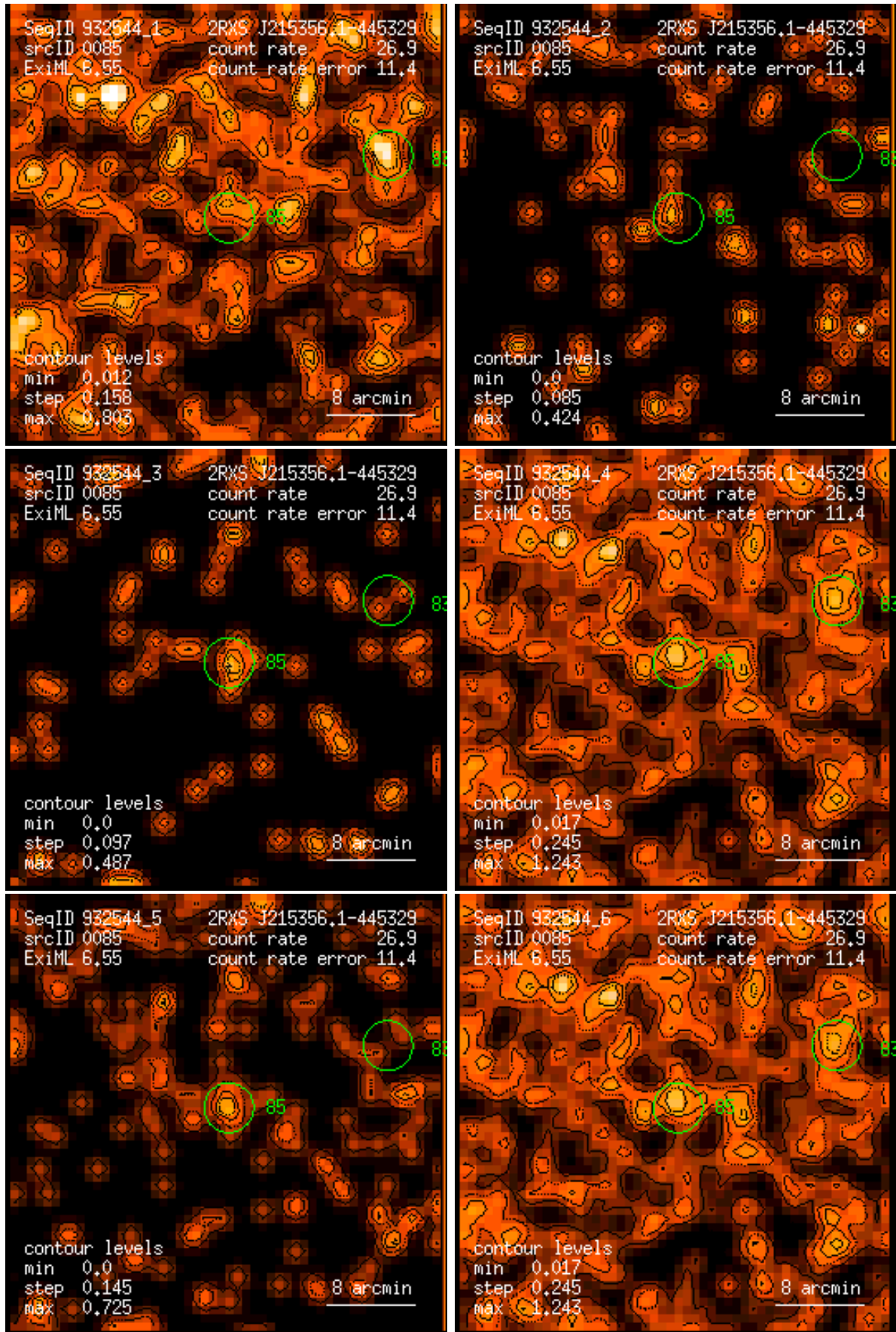
Figure 85: RASS 932544: detection 0085: band rate images, Gaussian filter: (1) PSPC channels 11 – 41, (2) 52 – 90, (3) 91 – 201, (4) 11 – 235, (5) 52 – 201, (6) 11 – 201. Broad band rates in counts/ks. Band rate contour levels in counts/ks/arcmin 2 .
