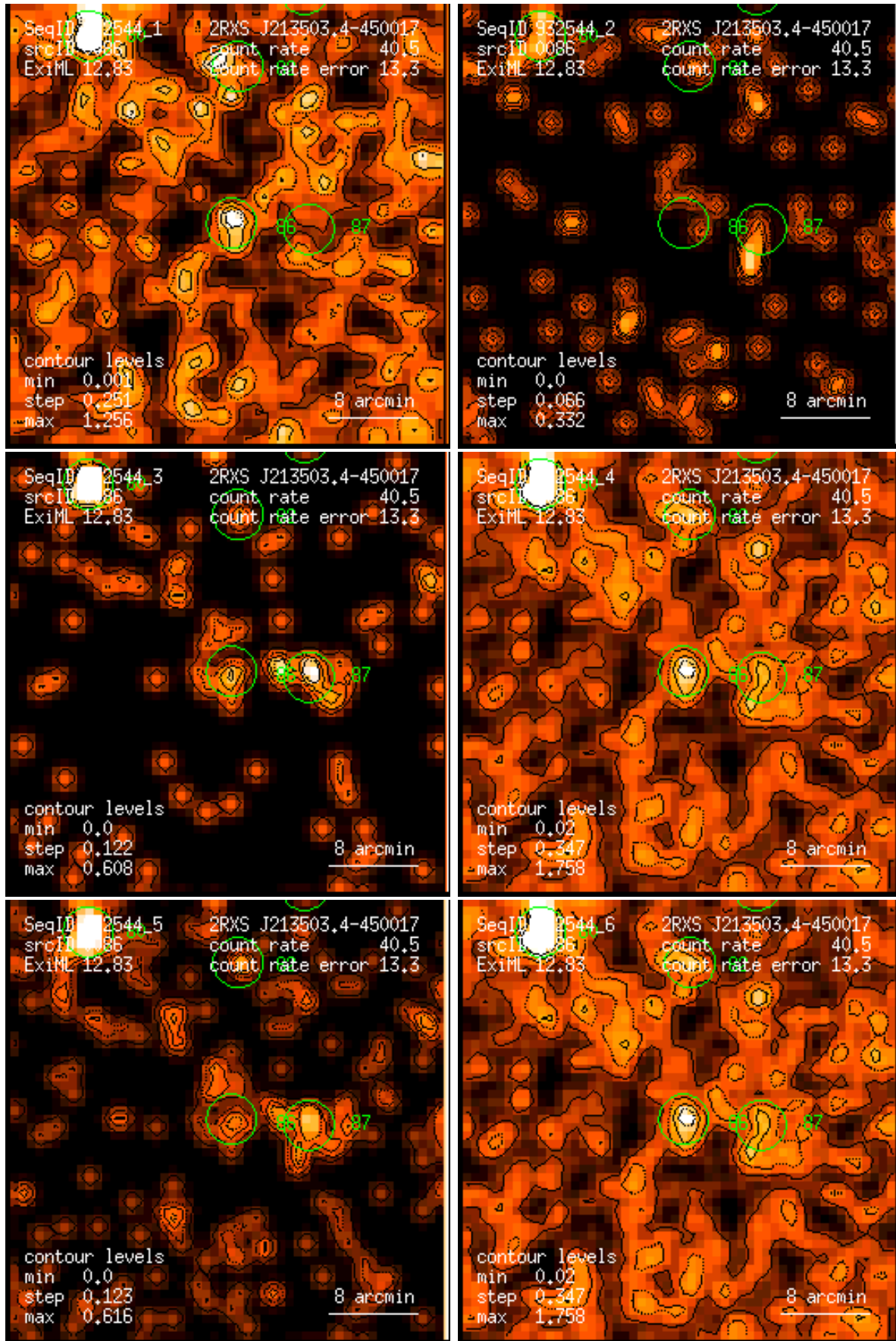
Figure 86: RASS 932544: detection 0086: band rate images, Gaussian filter: (1) PSPC channels 11 – 41, (2) 52 – 90, (3) 91 – 201, (4) 11 – 235, (5) 52 – 201, (6) 11 – 201. Broad band rates in counts/ks. Band rate contour levels in counts/ks/arcmin 2 .
