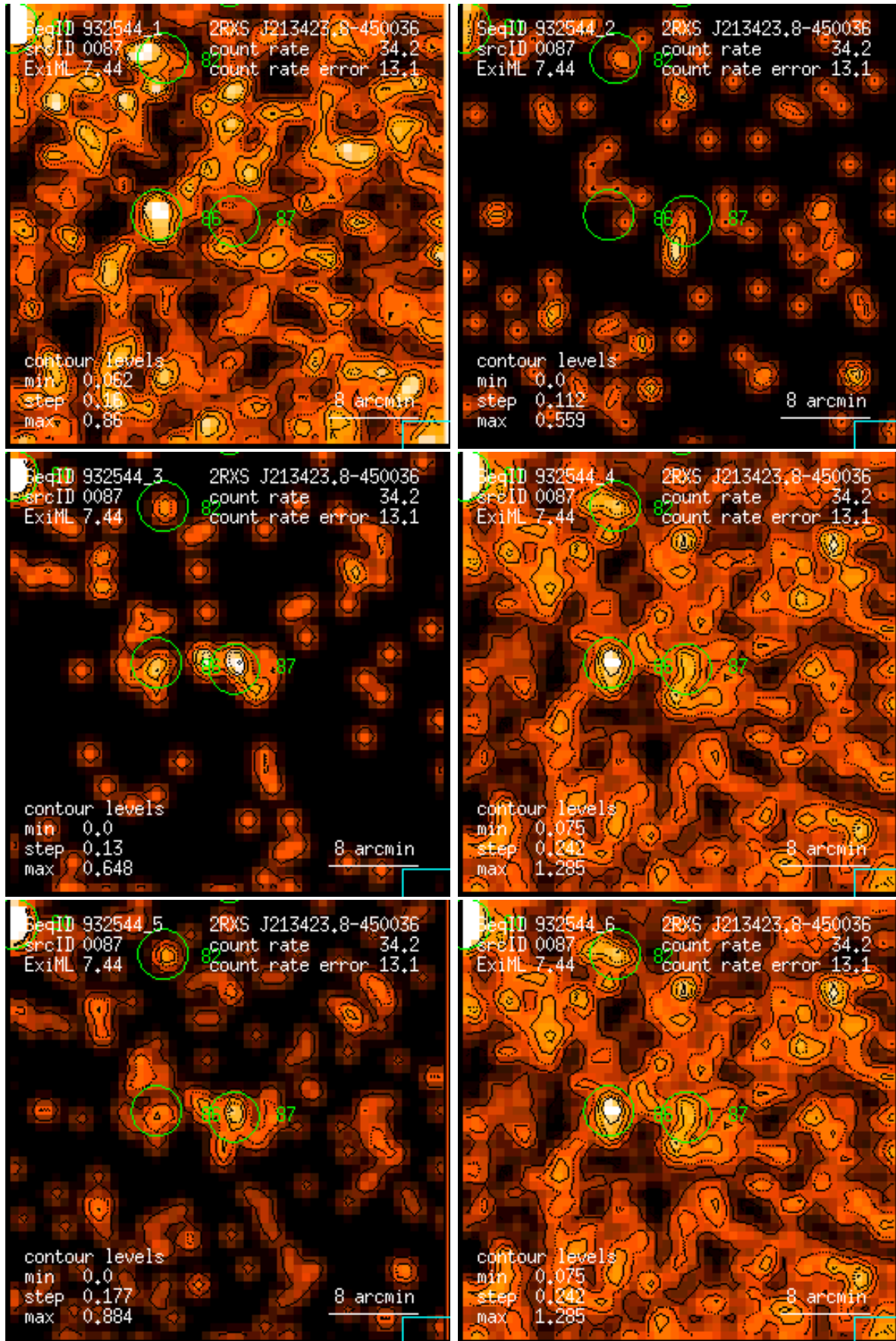
Figure 87: RASS 932544: detection 0087: band rate images, Gaussian filter: (1) PSPC channels 11 – 41, (2) 52 – 90, (3) 91 – 201, (4) 11 – 235, (5) 52 – 201, (6) 11 – 201. Broad band rates in counts/ks. Band rate contour levels in counts/ks/arcmin 2 .
