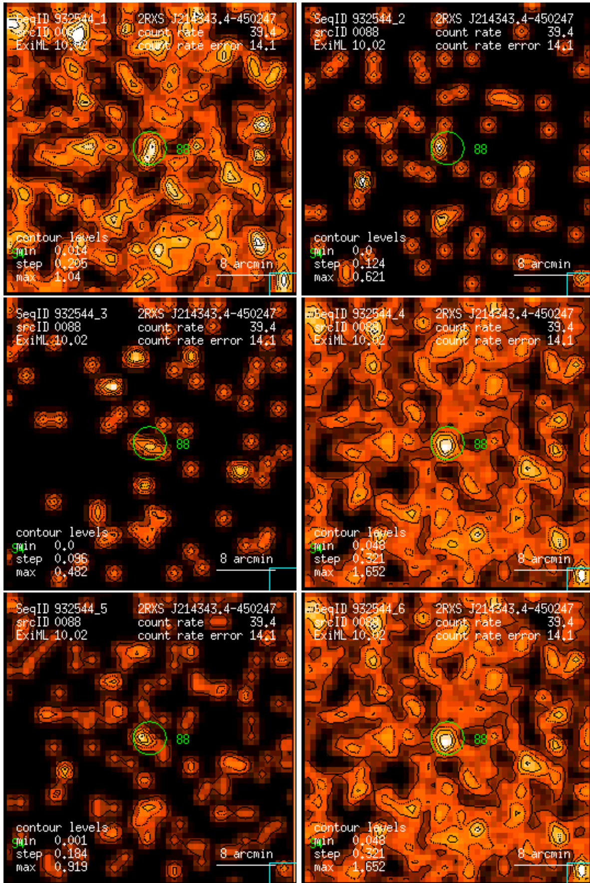
Figure 88: RASS 932544: detection 0088: band rate images, Gaussian filter: (1) PSPC channels 11 – 41, (2) 52 – 90, (3) 91 – 201, (4) 11 – 235, (5) 52 – 201, (6) 11 – 201. Broad band rates in counts/ks. Band rate contour levels in counts/ks/arcmin 2 .
