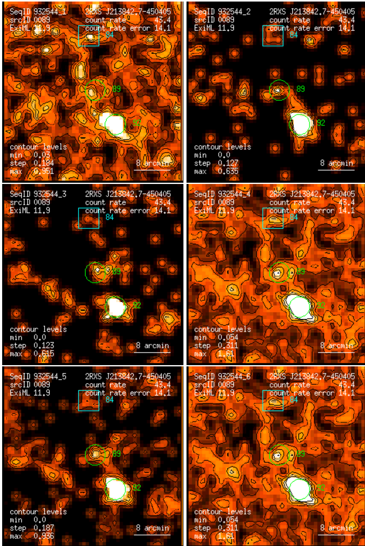
Figure 89: RASS 932544: detection 0089: band rate images, Gaussian filter: (1) PSPC channels 11 – 41, (2) 52 – 90, (3) 91 – 201, (4) 11 – 235, (5) 52 – 201, (6) 11 – 201. Broad band rates in counts/ks. Band rate contour levels in counts/ks/arcmin 2 .
