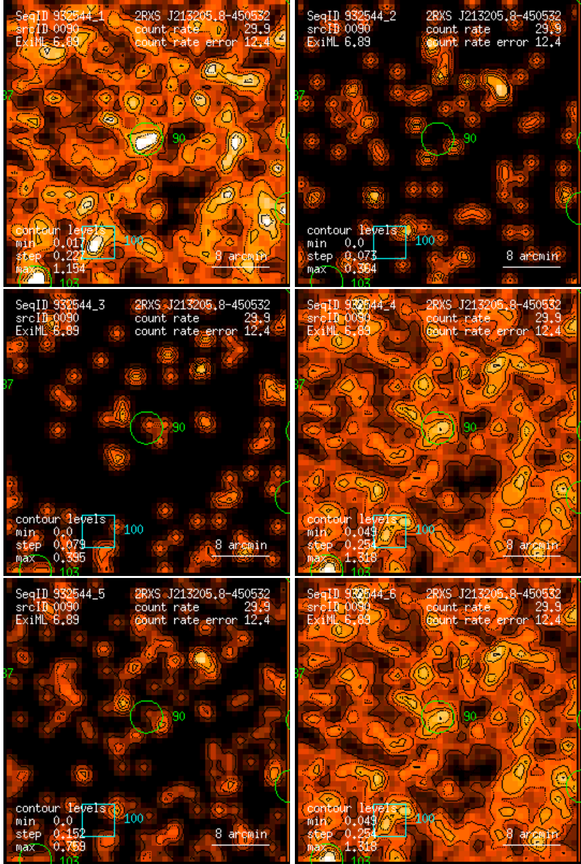
Figure 90: RASS 932544: detection 0090: band rate images, Gaussian filter: (1) PSPC channels 11 – 41, (2) 52 – 90, (3) 91 – 201, (4) 11 – 235, (5) 52 – 201, (6) 11 – 201. Broad band rates in counts/ks. Band rate contour levels in counts/ks/arcmin 2 .
