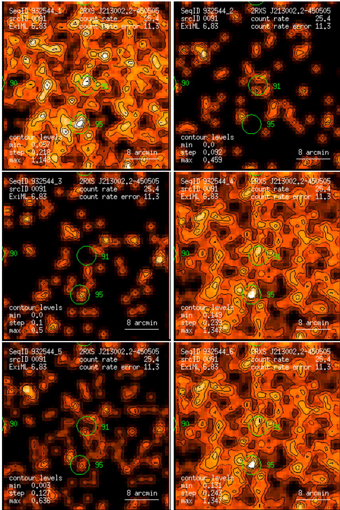
Figure 91: RASS 932544: detection 0091: band rate images, Gaussian filter: (1) PSPC channels 11 – 41, (2) 52 – 90, (3) 91 – 201, (4) 11 – 235, (5) 52 – 201, (6) 11 – 201. Broad band rates in counts/ks. Band rate contour levels in counts/ks/arcmin 2 .
