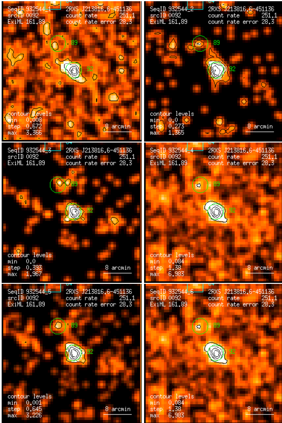
Figure 92: RASS 932544: detection 0092: band rate images, Gaussian filter: (1) PSPC channels 11 – 41, (2) 52 – 90, (3) 91 – 201, (4) 11 – 235, (5) 52 – 201, (6) 11 – 201. Broad band rates in counts/ks. Band rate contour levels in counts/ks/arcmin 2 .
