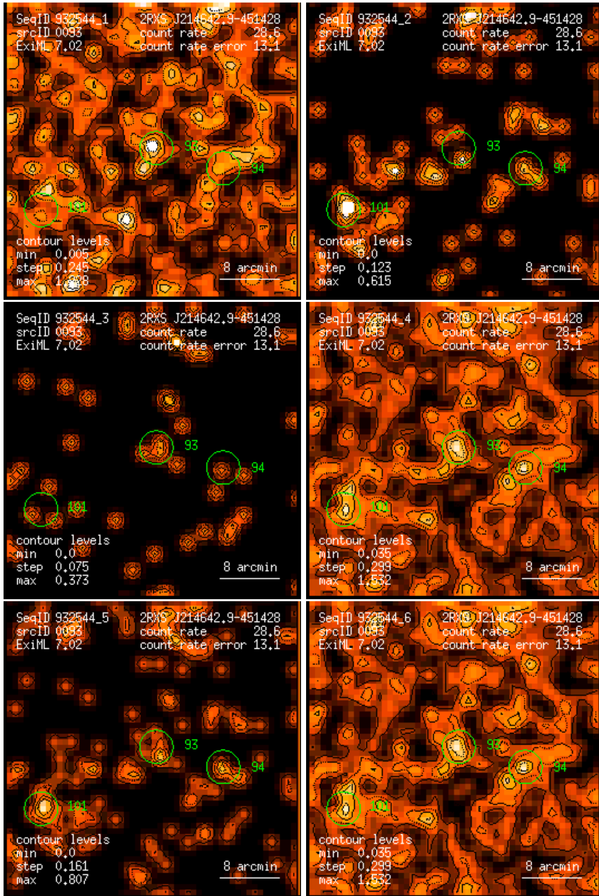
Figure 93: RASS 932544: detection 0093: band rate images, Gaussian filter: (1) PSPC channels 11 – 41, (2) 52 – 90, (3) 91 – 201, (4) 11 – 235, (5) 52 – 201, (6) 11 – 201. Broad band rates in counts/ks. Band rate contour levels in counts/ks/arcmin 2 .
