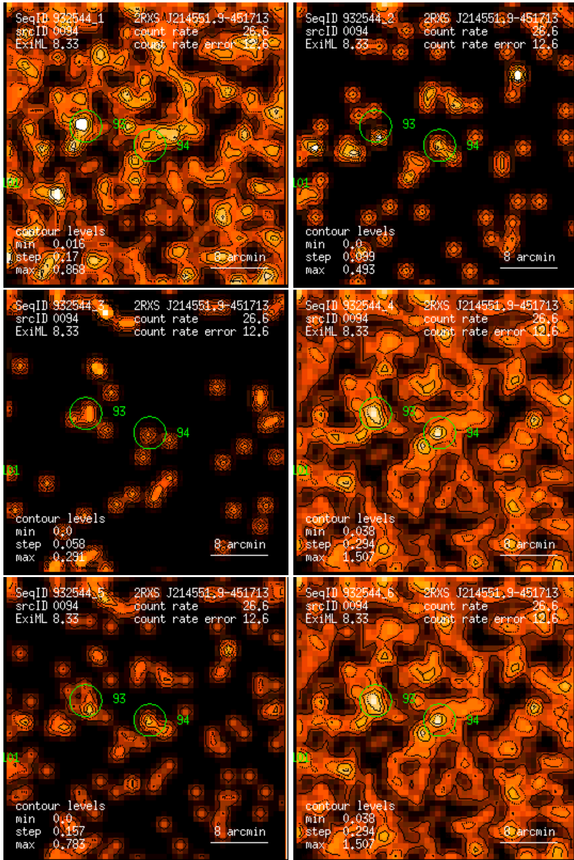
Figure 94: RASS 932544: detection 0094: band rate images, Gaussian filter: (1) PSPC channels 11 – 41, (2) 52 – 90, (3) 91 – 201, (4) 11 – 235, (5) 52 – 201, (6) 11 – 201. Broad band rates in counts/ks. Band rate contour levels in counts/ks/arcmin 2 .
