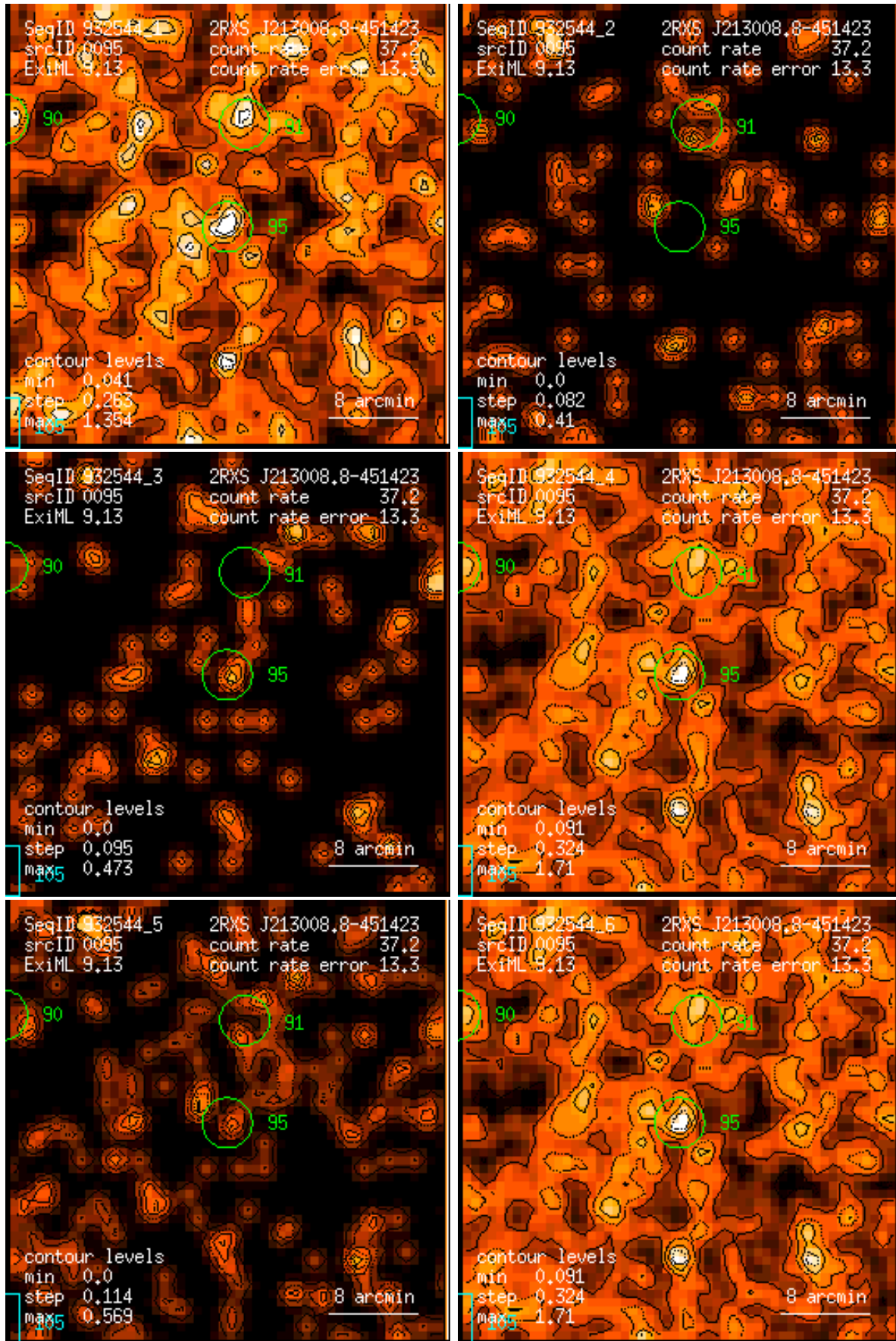
Figure 95: RASS 932544: detection 0095: band rate images, Gaussian filter: (1) PSPC channels 11 – 41, (2) 52 – 90, (3) 91 – 201, (4) 11 – 235, (5) 52 – 201, (6) 11 – 201. Broad band rates in counts/ks. Band rate contour levels in counts/ks/arcmin 2 .
