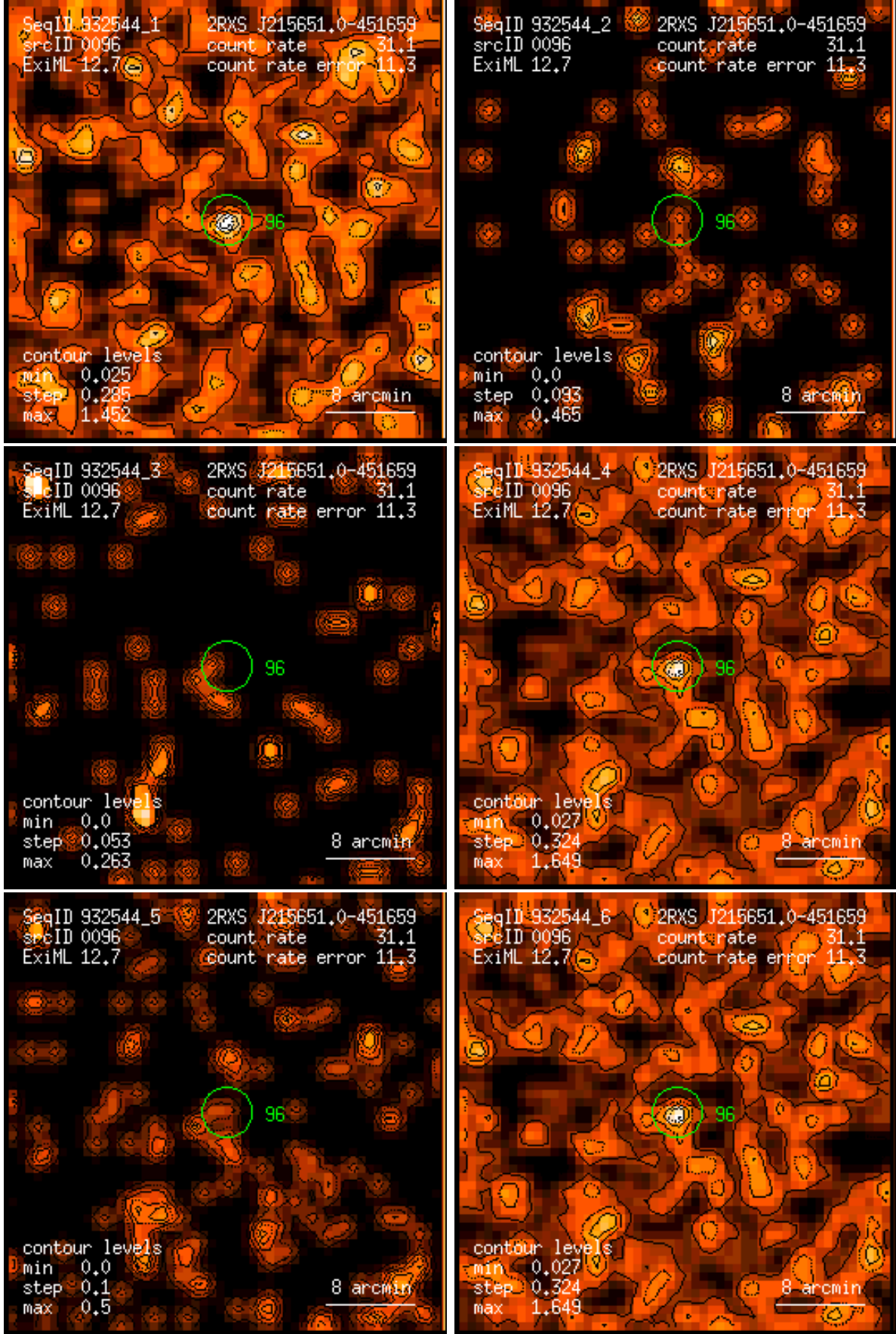
Figure 96: RASS 932544: detection 0096: band rate images, Gaussian filter: (1) PSPC channels 11 – 41, (2) 52 – 90, (3) 91 – 201, (4) 11 – 235, (5) 52 – 201, (6) 11 – 201. Broad band rates in counts/ks. Band rate contour levels in counts/ks/arcmin 2 .
