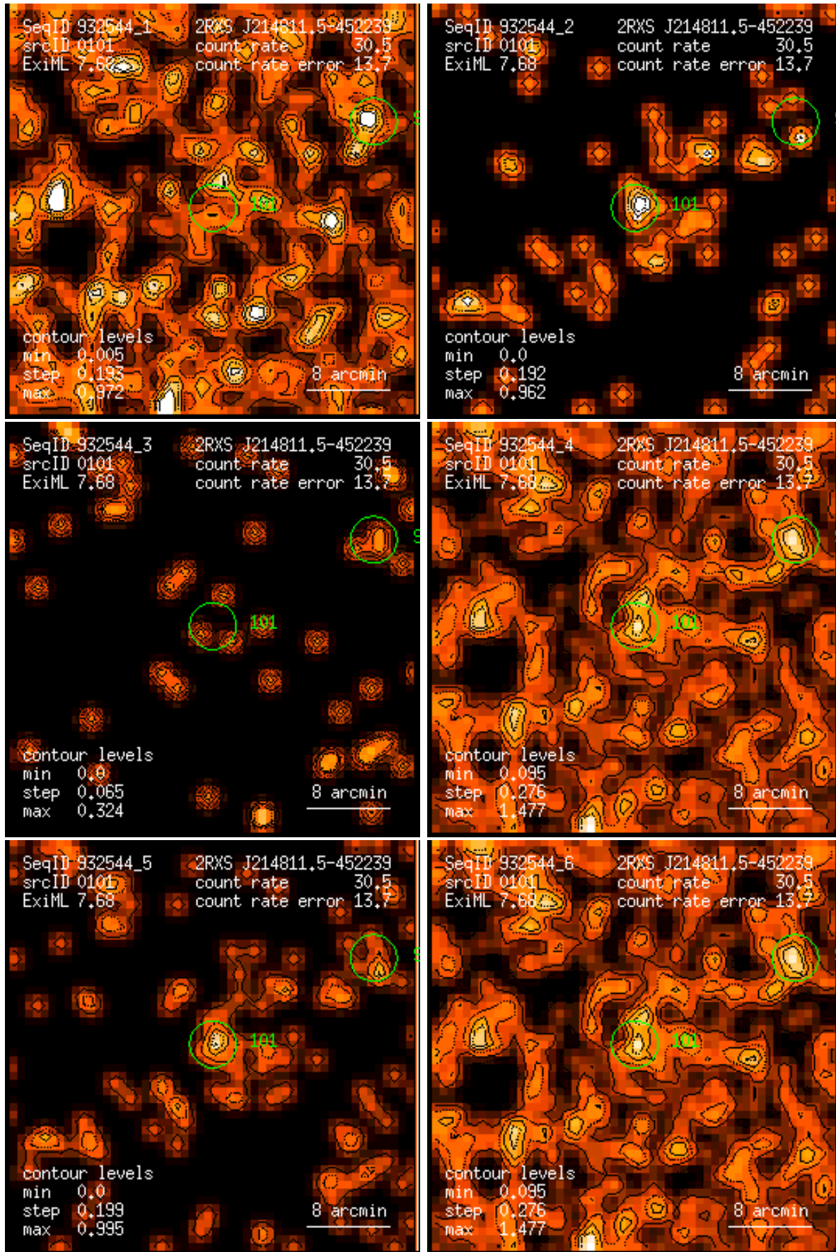
Figure 101: RASS 932544: detection 0101: band rate images, Gaussian filter: (1) PSPC channels 11 – 41, (2) 52 – 90, (3) 91 – 201, (4) 11 – 235, (5) 52 – 201, (6) 11 – 201. Broad band rates in counts/ks. Band rate contour levels in counts/ks/arcmin 2 .
