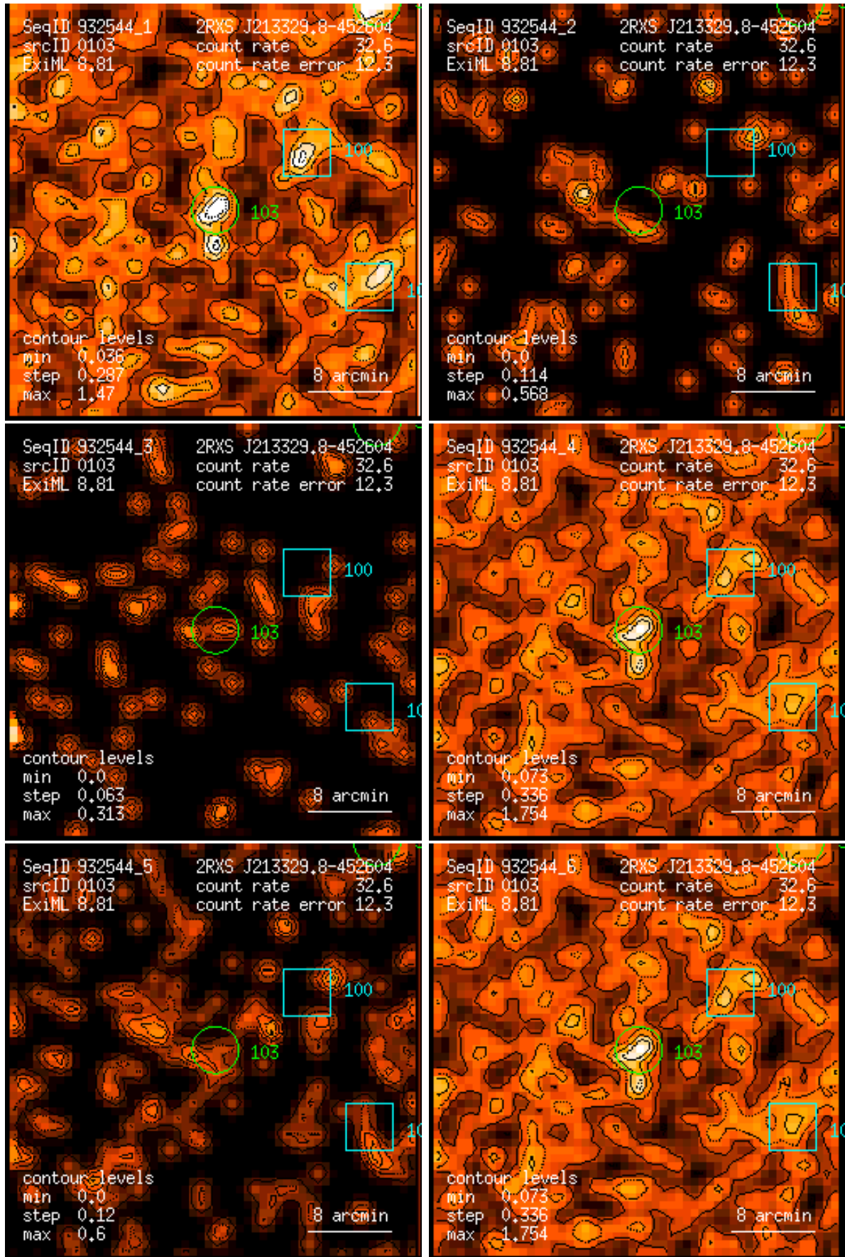
Figure 103: RASS 932544: detection 0103: band rate images, Gaussian filter: (1) PSPC channels 11 – 41, (2) 52 – 90, (3) 91 – 201, (4) 11 – 235, (5) 52 – 201, (6) 11 – 201. Broad band rates in counts/ks. Band rate contour levels in counts/ks/arcmin 2 .
