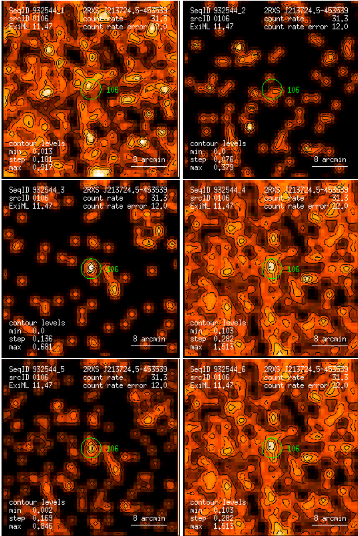
Figure 106: RASS 932544: detection 0106: band rate images, Gaussian filter: (1) PSPC channels 11 – 41, (2) 52 – 90, (3) 91 – 201, (4) 11 – 235, (5) 52 – 201, (6) 11 – 201. Broad band rates in counts/ks. Band rate contour levels in counts/ks/arcmin 2 .
