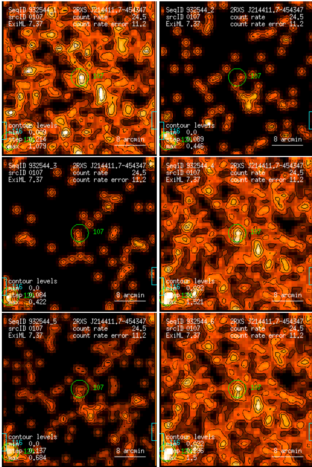
Figure 107: RASS 932544: detection 0107: band rate images, Gaussian filter: (1) PSPC channels 11 – 41, (2) 52 – 90, (3) 91 – 201, (4) 11 – 235, (5) 52 – 201, (6) 11 – 201. Broad band rates in counts/ks. Band rate contour levels in counts/ks/arcmin 2 .
