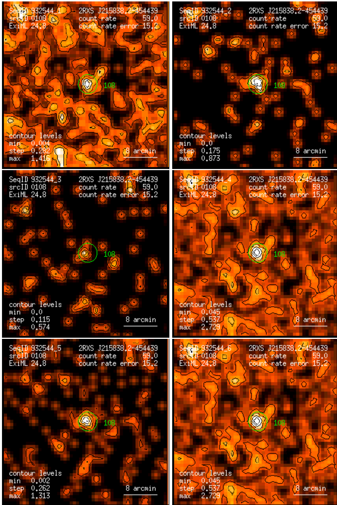
Figure 108: RASS 932544: detection 0108: band rate images, Gaussian filter: (1) PSPC channels 11 – 41, (2) 52 – 90, (3) 91 – 201, (4) 11 – 235, (5) 52 – 201, (6) 11 – 201. Broad band rates in counts/ks. Band rate contour levels in counts/ks/arcmin 2 .
