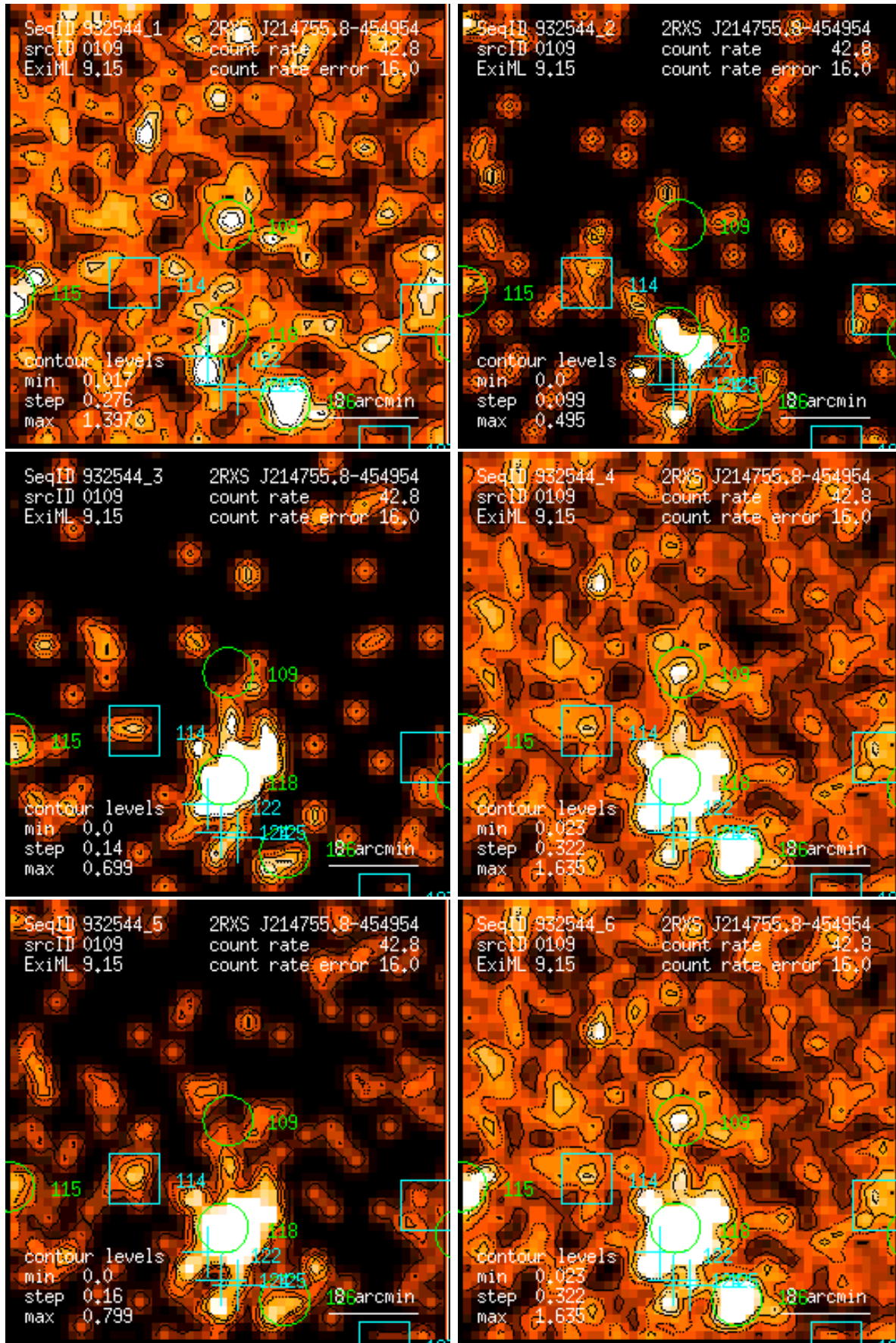
Figure 109: RASS 932544: detection 0109: band rate images, Gaussian filter: (1) PSPC channels 11 – 41, (2) 52 – 90, (3) 91 – 201, (4) 11 – 235, (5) 52 – 201, (6) 11 – 201. Broad band rates in counts/ks. Band rate contour levels in counts/ks/arcmin 2 .
