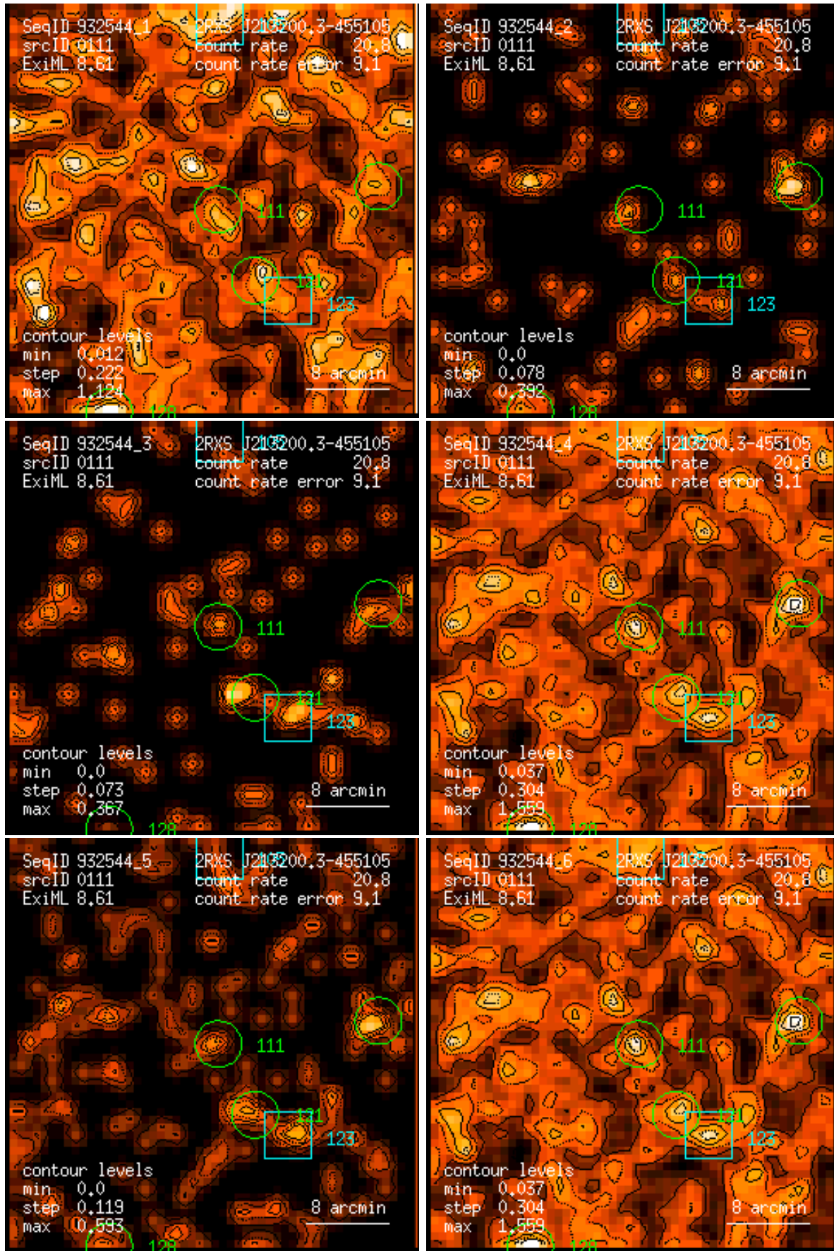
Figure 111: RASS 932544: detection 0111: band rate images, Gaussian filter: (1) PSPC channels 11 – 41, (2) 52 – 90, (3) 91 – 201, (4) 11 – 235, (5) 52 – 201, (6) 11 – 201. Broad band rates in counts/ks. Band rate contour levels in counts/ks/arcmin 2 .
