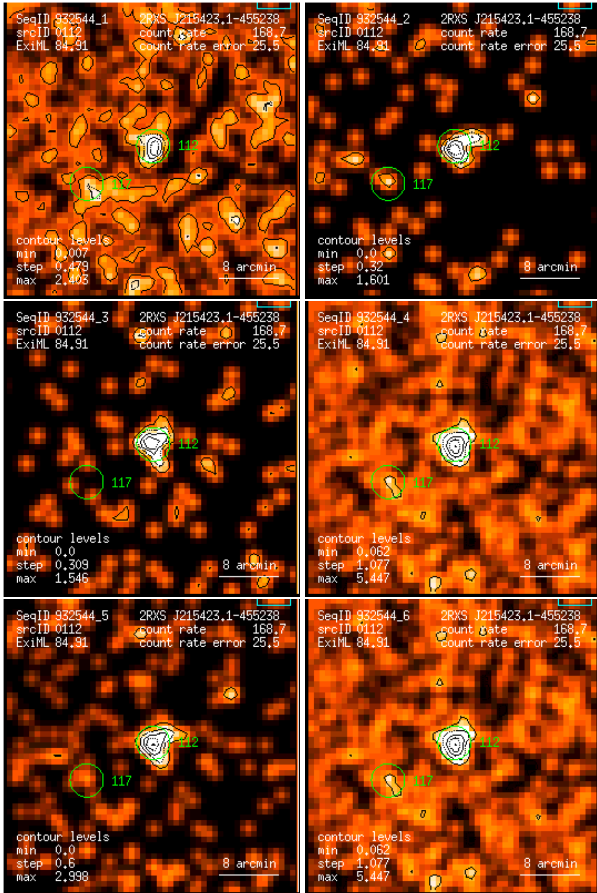
Figure 112: RASS 932544: detection 0112: band rate images, Gaussian filter: (1) PSPC channels 11 – 41, (2) 52 – 90, (3) 91 – 201, (4) 11 – 235, (5) 52 – 201, (6) 11 – 201. Broad band rates in counts/ks. Band rate contour levels in counts/ks/arcmin 2 .
