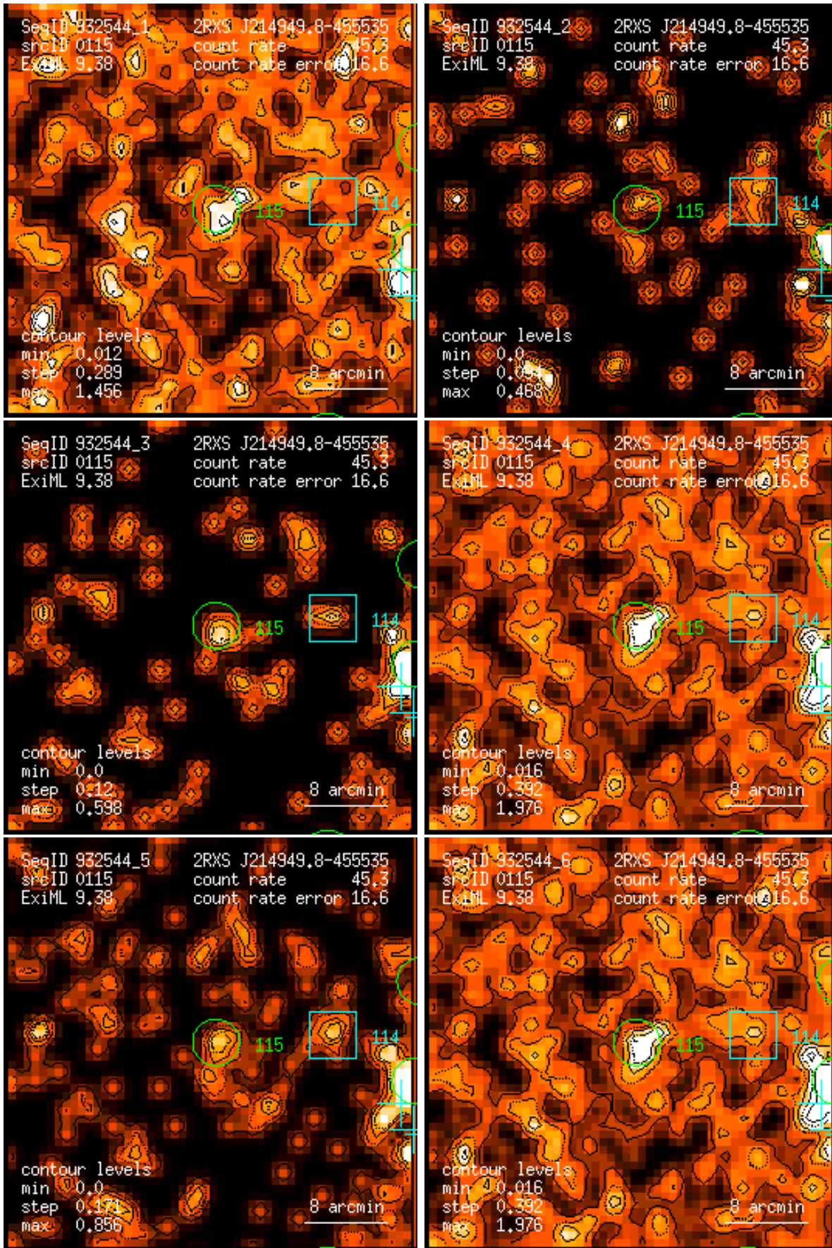
Figure 115: RASS 932544: detection 0115: band rate images, Gaussian filter: (1) PSPC channels 11 – 41, (2) 52 – 90, (3) 91 – 201, (4) 11 – 235, (5) 52 – 201, (6) 11 – 201. Broad band rates in counts/ks. Band rate contour levels in counts/ks/arcmin 2 .
