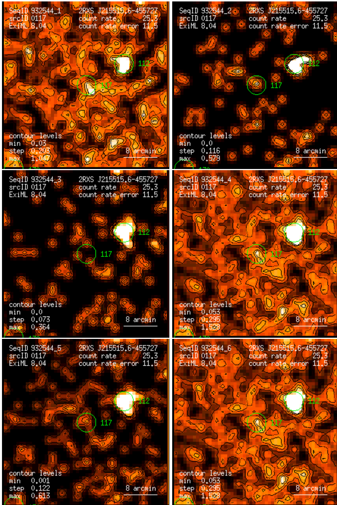
Figure 117: RASS 932544: detection 0117: band rate images, Gaussian filter: (1) PSPC channels 11 – 41, (2) 52 – 90, (3) 91 – 201, (4) 11 – 235, (5) 52 – 201, (6) 11 – 201. Broad band rates in counts/ks. Band rate contour levels in counts/ks/arcmin 2 .
