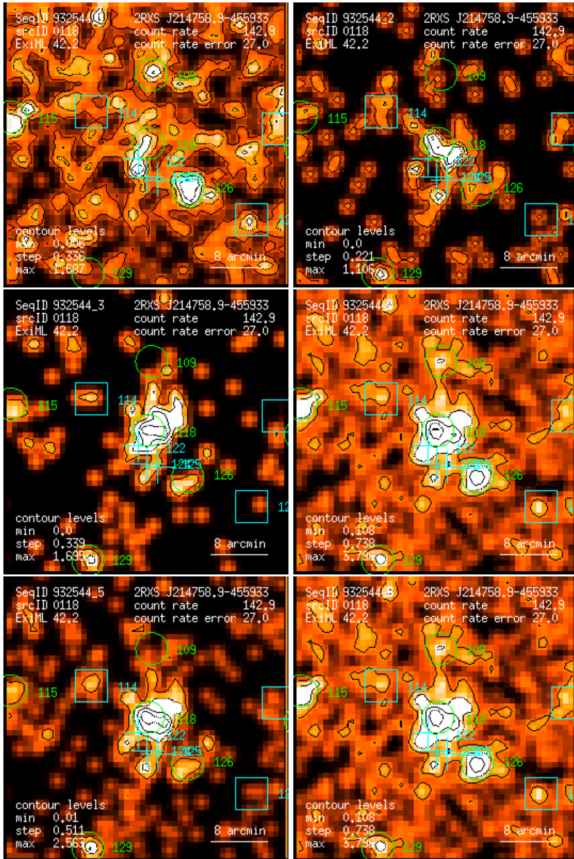
Figure 118: RASS 932544: detection 0118: band rate images, Gaussian filter: (1) PSPC channels 11 – 41, (2) 52 – 90, (3) 91 – 201, (4) 11 – 235, (5) 52 – 201, (6) 11 – 201. Broad band rates in counts/ks. Band rate contour levels in counts/ks/arcmin 2 .
