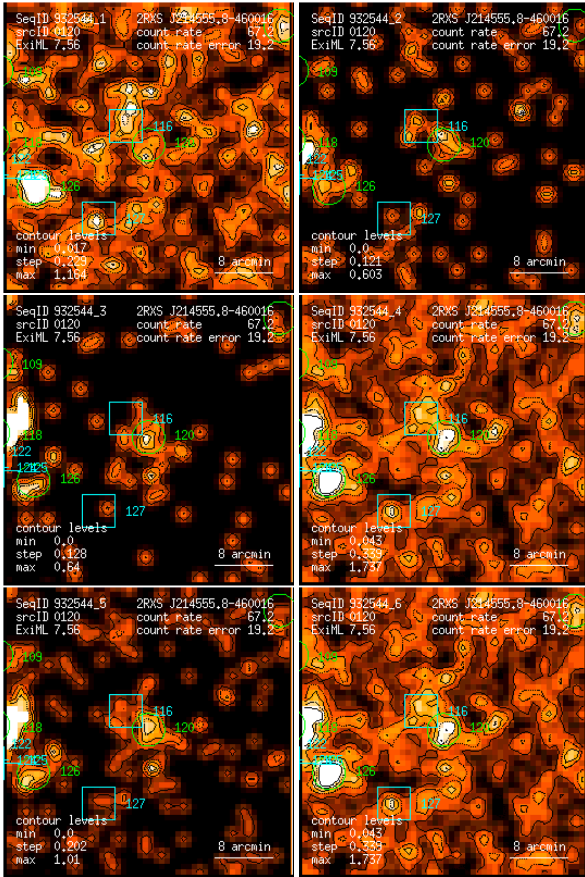
Figure 120: RASS 932544: detection 0120: band rate images, Gaussian filter: (1) PSPC channels 11 – 41, (2) 52 – 90, (3) 91 – 201, (4) 11 – 235, (5) 52 – 201, (6) 11 – 201. Broad band rates in counts/ks. Band rate contour levels in counts/ks/arcmin 2 .
