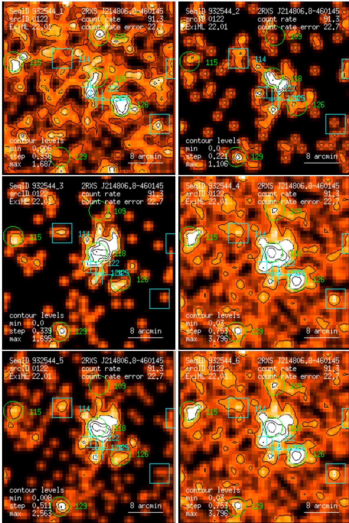
Figure 122: RASS 932544: detection 0122: band rate images, Gaussian filter: (1) PSPC channels 11 – 41, (2) 52 – 90, (3) 91 – 201, (4) 11 – 235, (5) 52 – 201, (6) 11 – 201. Broad band rates in counts/ks. Band rate contour levels in counts/ks/arcmin 2 .
