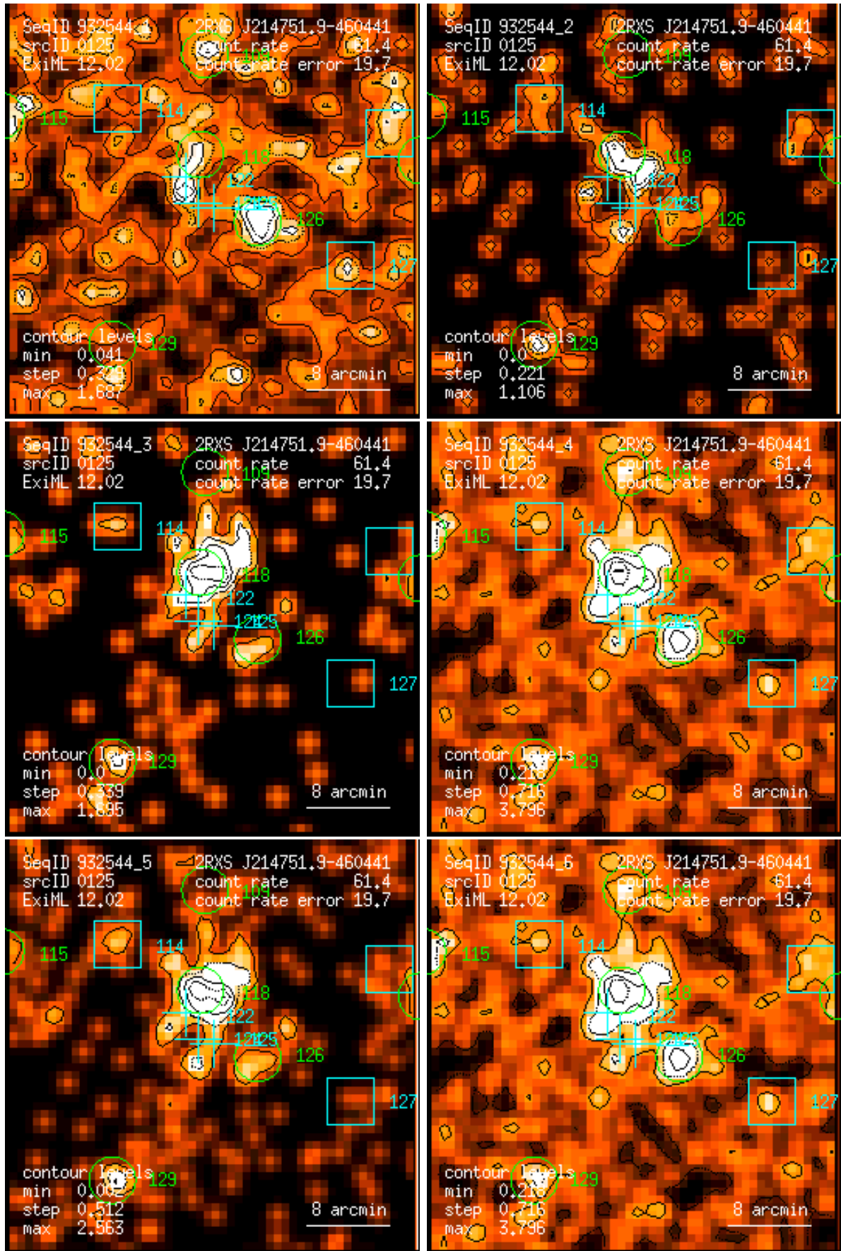
Figure 125: RASS 932544: detection 0125: band rate images, Gaussian filter: (1) PSPC channels 11 – 41, (2) 52 – 90, (3) 91 – 201, (4) 11 – 235, (5) 52 – 201, (6) 11 – 201. Broad band rates in counts/ks. Band rate contour levels in counts/ks/arcmin 2 .
