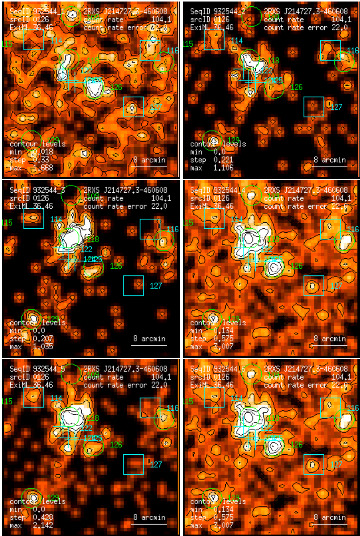
Figure 126: RASS 932544: detection 0126: band rate images, Gaussian filter: (1) PSPC channels 11 – 41, (2) 52 – 90, (3) 91 – 201, (4) 11 – 235, (5) 52 – 201, (6) 11 – 201. Broad band rates in counts/ks. Band rate contour levels in counts/ks/arcmin 2 .
