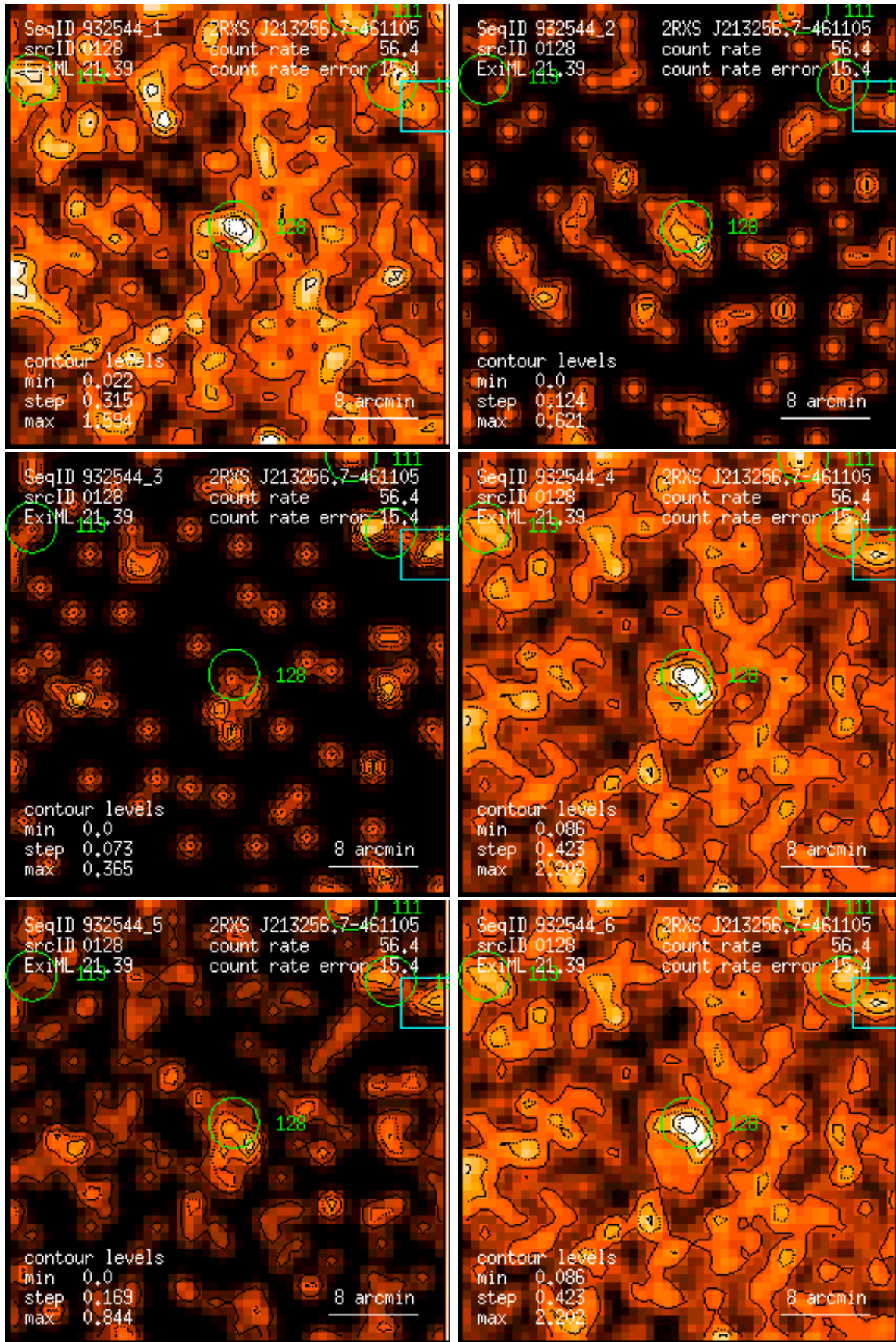
Figure 128: RASS 932544: detection 0128: band rate images, Gaussian filter: (1) PSPC channels 11 – 41, (2) 52 – 90, (3) 91 – 201, (4) 11 – 235, (5) 52 – 201, (6) 11 – 201. Broad band rates in counts/ks. Band rate contour levels in counts/ks/arcmin 2 .
