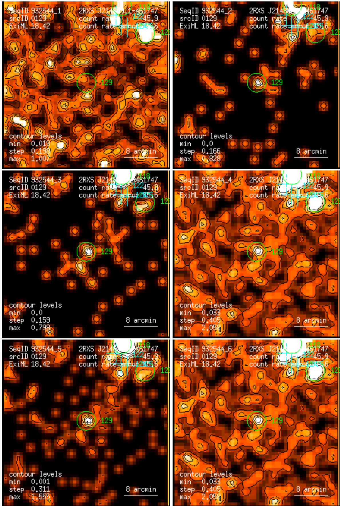
Figure 129: RASS 932544: detection 0129: band rate images, Gaussian filter: (1) PSPC channels 11 – 41, (2) 52 – 90, (3) 91 – 201, (4) 11 – 235, (5) 52 – 201, (6) 11 – 201. Broad band rates in counts/ks. Band rate contour levels in counts/ks/arcmin 2 .
