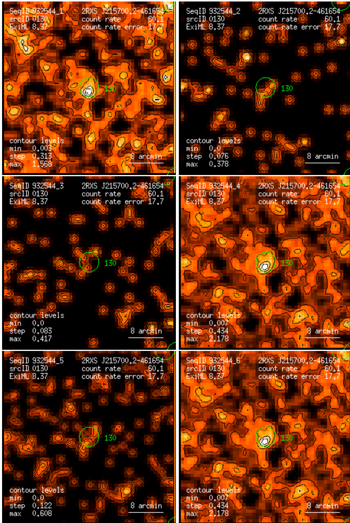
Figure 130: RASS 932544: detection 0130: band rate images, Gaussian filter: (1) PSPC channels 11 – 41, (2) 52 – 90, (3) 91 – 201, (4) 11 – 235, (5) 52 – 201, (6) 11 – 201. Broad band rates in counts/ks. Band rate contour levels in counts/ks/arcmin 2 .
